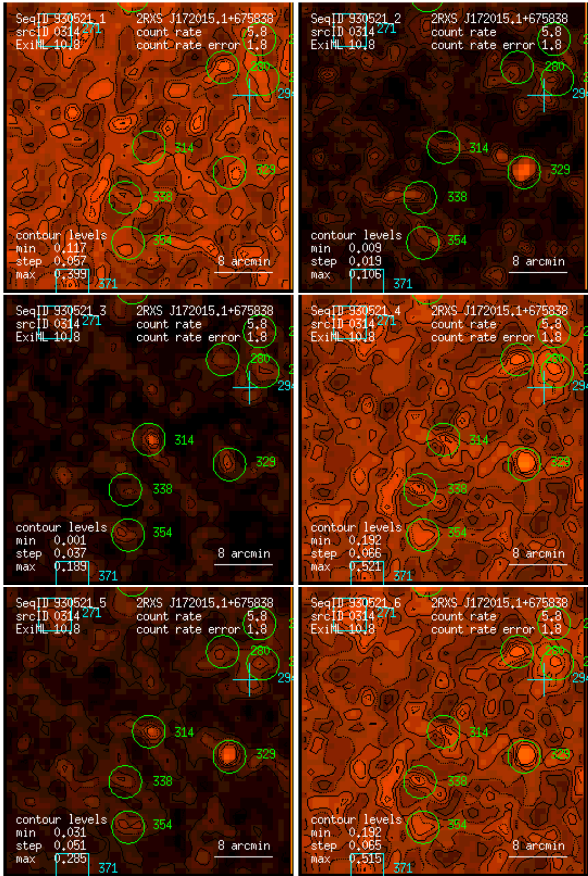
Figure 314: RASS 930521: detection 0314: band rate images, Gaussian filter: (1) PSPC channels 11 – 41, (2) 52 – 90, (3) 91 – 201, (4) 11 – 235, (5) 52 – 201, (6) 11 – 201. Broad band rates in counts/ks. Band rate contour levels in counts/ks/arcmin 2 .
