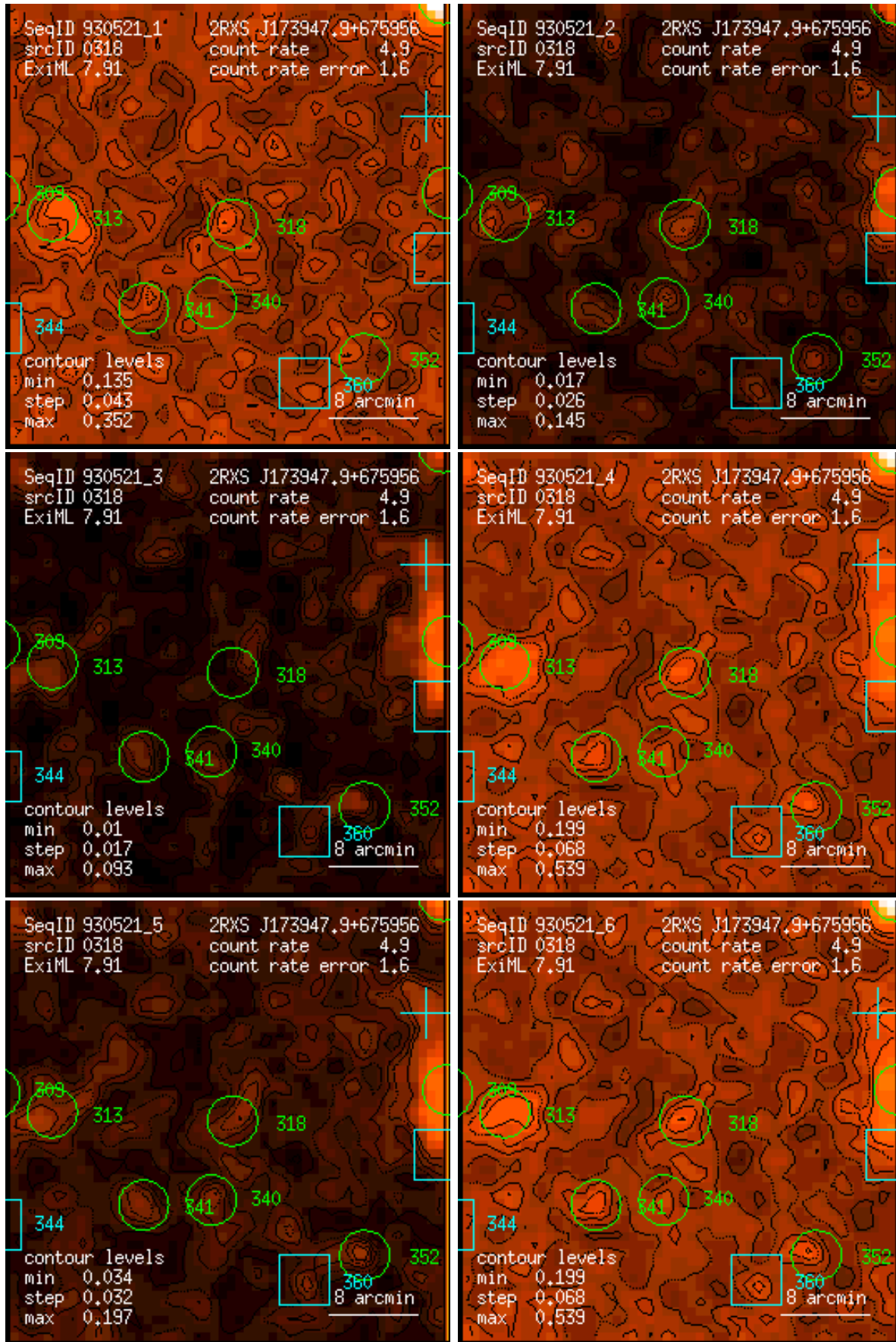
Figure 318: RASS 930521: detection 0318: band rate images, Gaussian filter: (1) PSPC channels 11 – 41, (2) 52 – 90, (3) 91 – 201, (4) 11 – 235, (5) 52 – 201, (6) 11 – 201. Broad band rates in counts/ks. Band rate contour levels in counts/ks/arcmin 2 .
