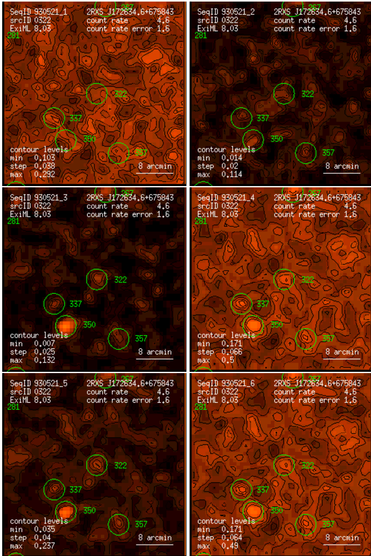
Figure 322: RASS 930521: detection 0322: band rate images, Gaussian filter: (1) PSPC channels 11 – 41, (2) 52 – 90, (3) 91 – 201, (4) 11 – 235, (5) 52 – 201, (6) 11 – 201. Broad band rates in counts/ks. Band rate contour levels in counts/ks/arcmin 2 .
