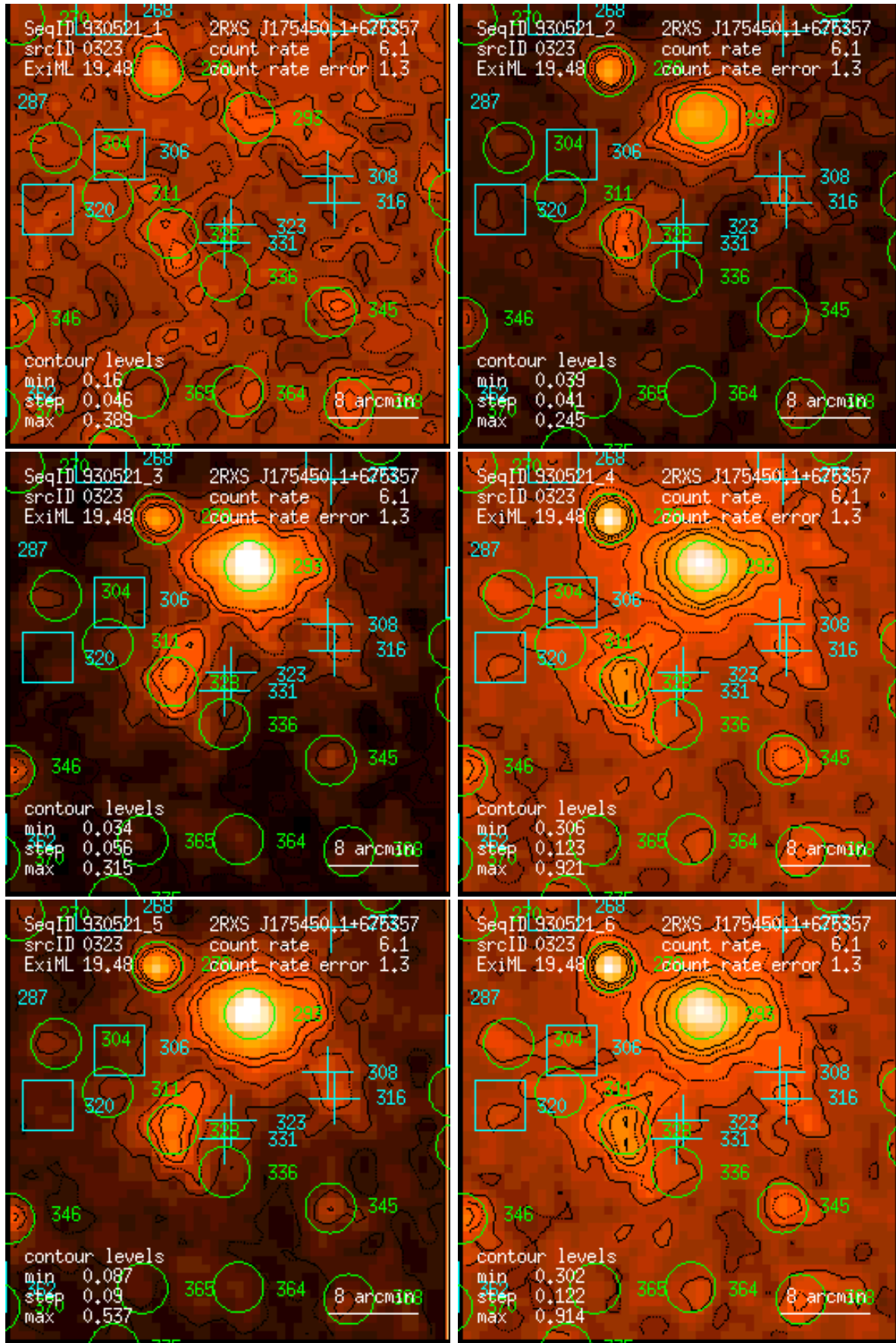
Figure 323: RASS 930521: detection 0323: band rate images, Gaussian filter: (1) PSPC channels 11 – 41, (2) 52 – 90, (3) 91 – 201, (4) 11 – 235, (5) 52 – 201, (6) 11 – 201. Broad band rates in counts/ks. Band rate contour levels in counts/ks/arcmin 2 .
