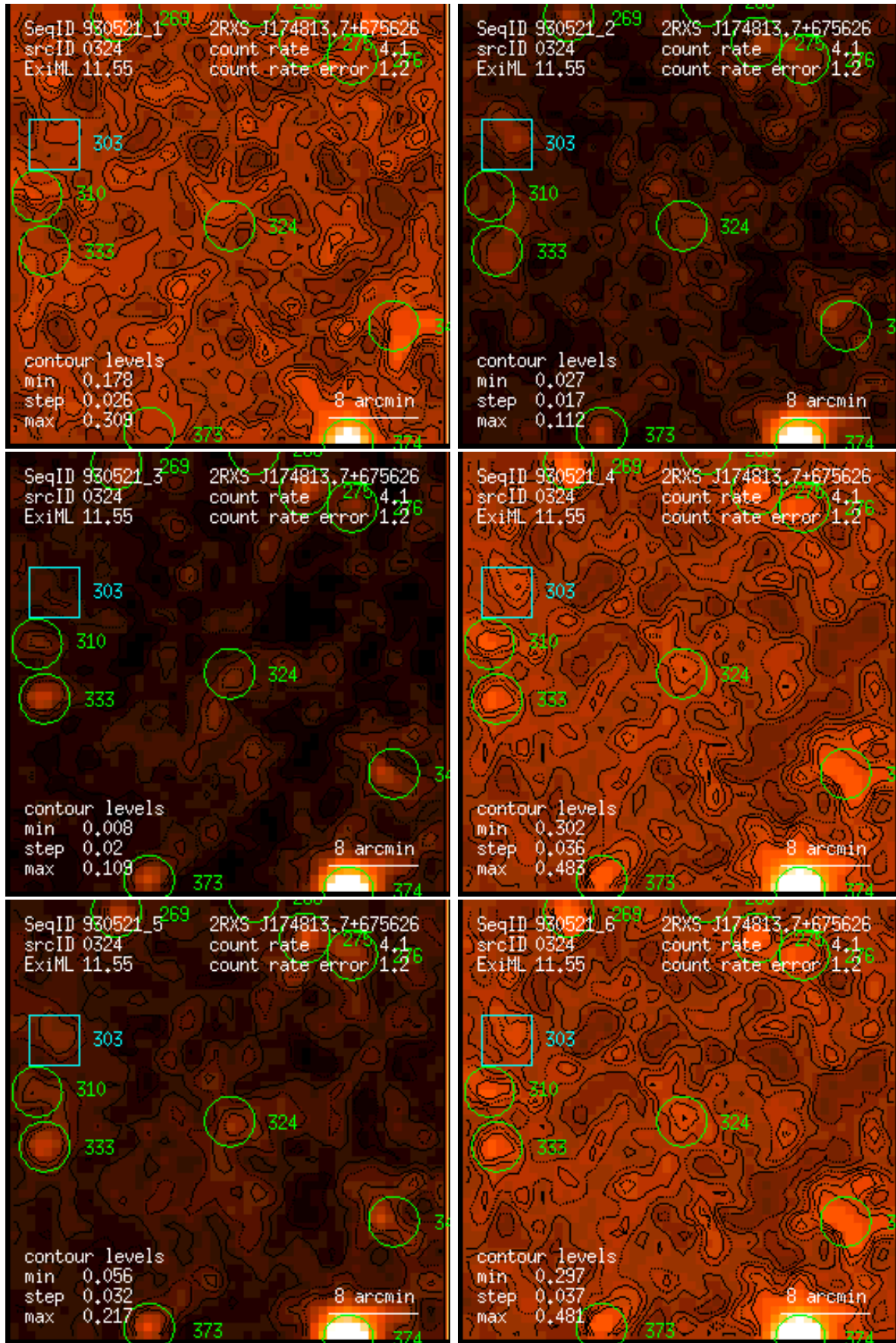
Figure 324: RASS 930521: detection 0324: band rate images, Gaussian filter: (1) PSPC channels 11 – 41, (2) 52 – 90, (3) 91 – 201, (4) 11 – 235, (5) 52 – 201, (6) 11 – 201. Broad band rates in counts/ks. Band rate contour levels in counts/ks/arcmin 2 .
