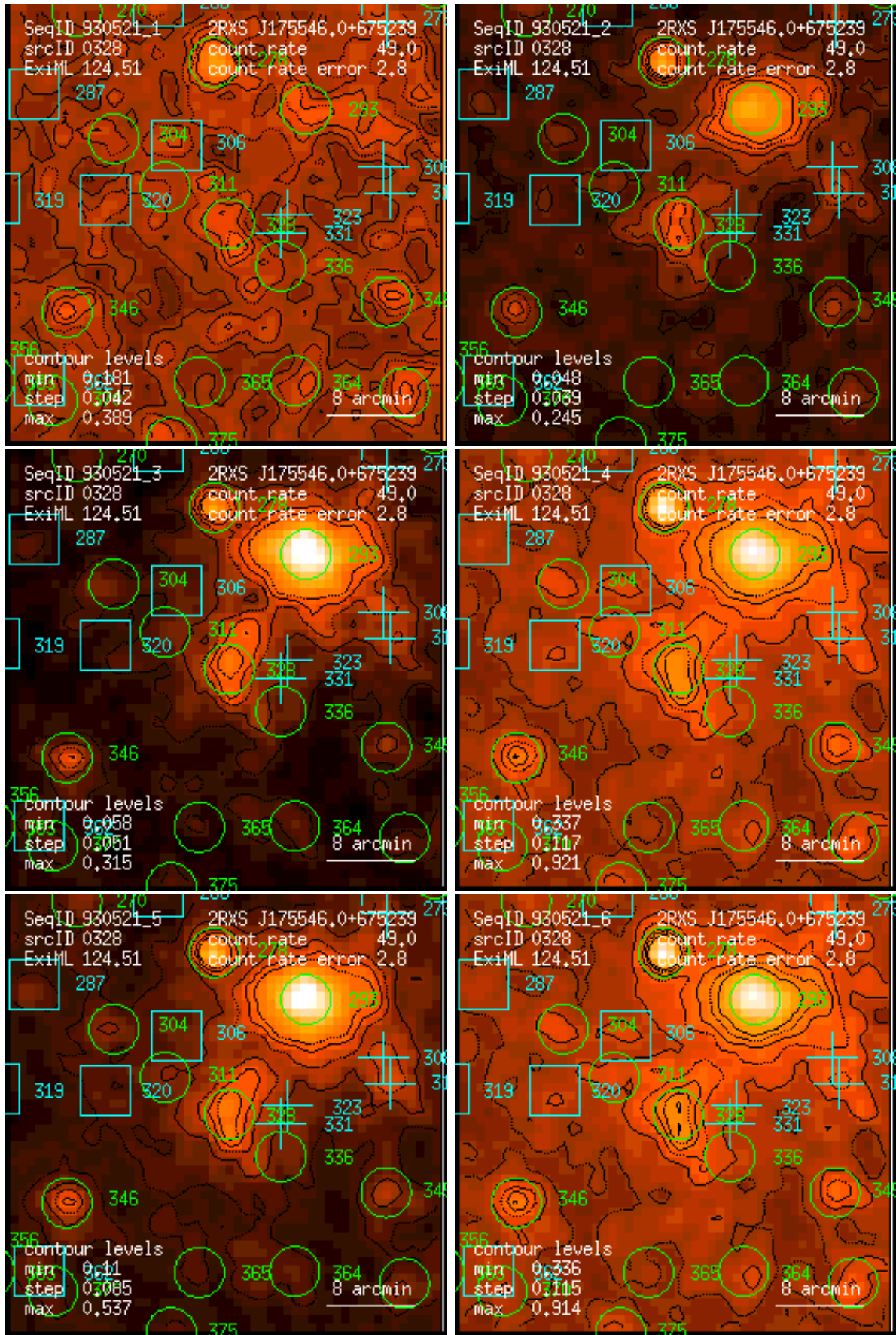
Figure 328: RASS 930521: detection 0328: band rate images, Gaussian filter: (1) PSPC channels 11 – 41, (2) 52 – 90, (3) 91 – 201, (4) 11 – 235, (5) 52 – 201, (6) 11 – 201. Broad band rates in counts/ks. Band rate contour levels in counts/ks/arcmin 2 .
