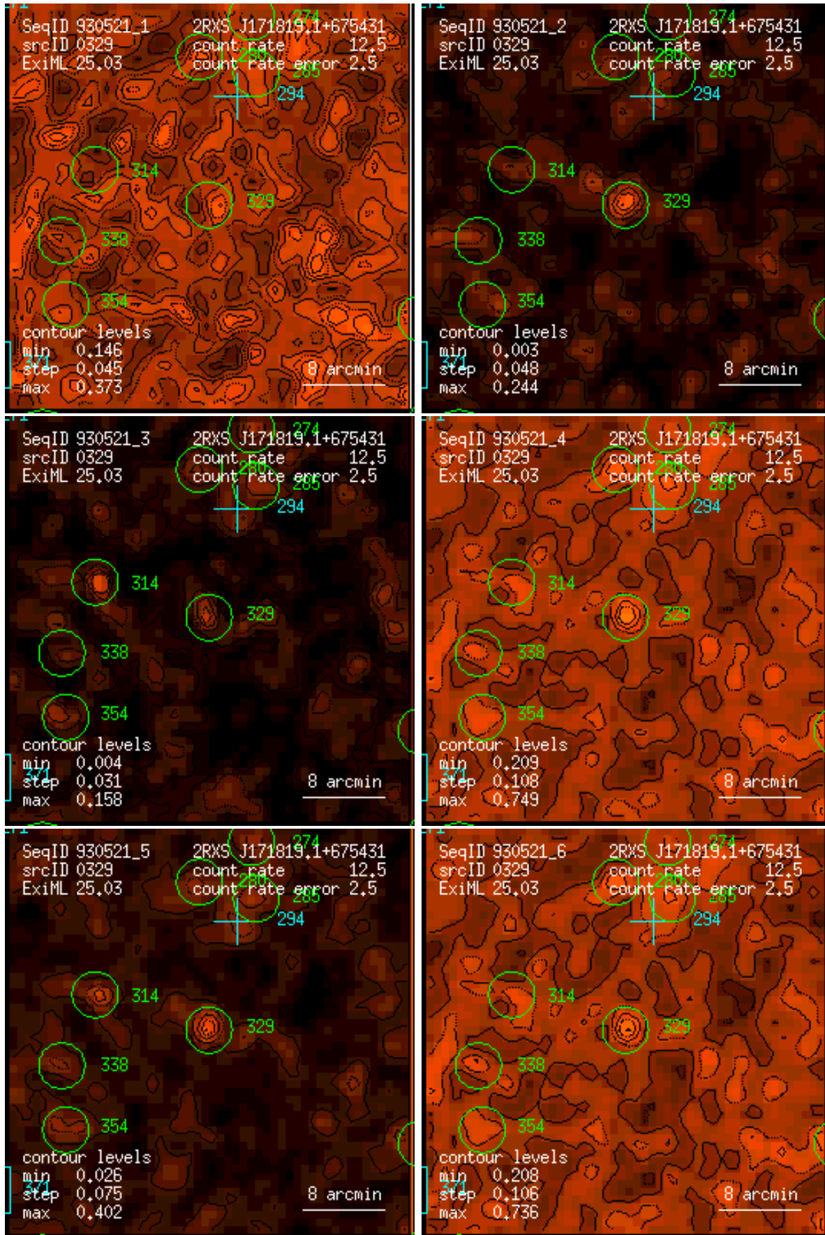
Figure 329: RASS 930521: detection 0329: band rate images, Gaussian filter: (1) PSPC channels 11 – 41, (2) 52 – 90, (3) 91 – 201, (4) 11 – 235, (5) 52 – 201, (6) 11 – 201. Broad band rates in counts/ks. Band rate contour levels in counts/ks/arcmin 2 .
