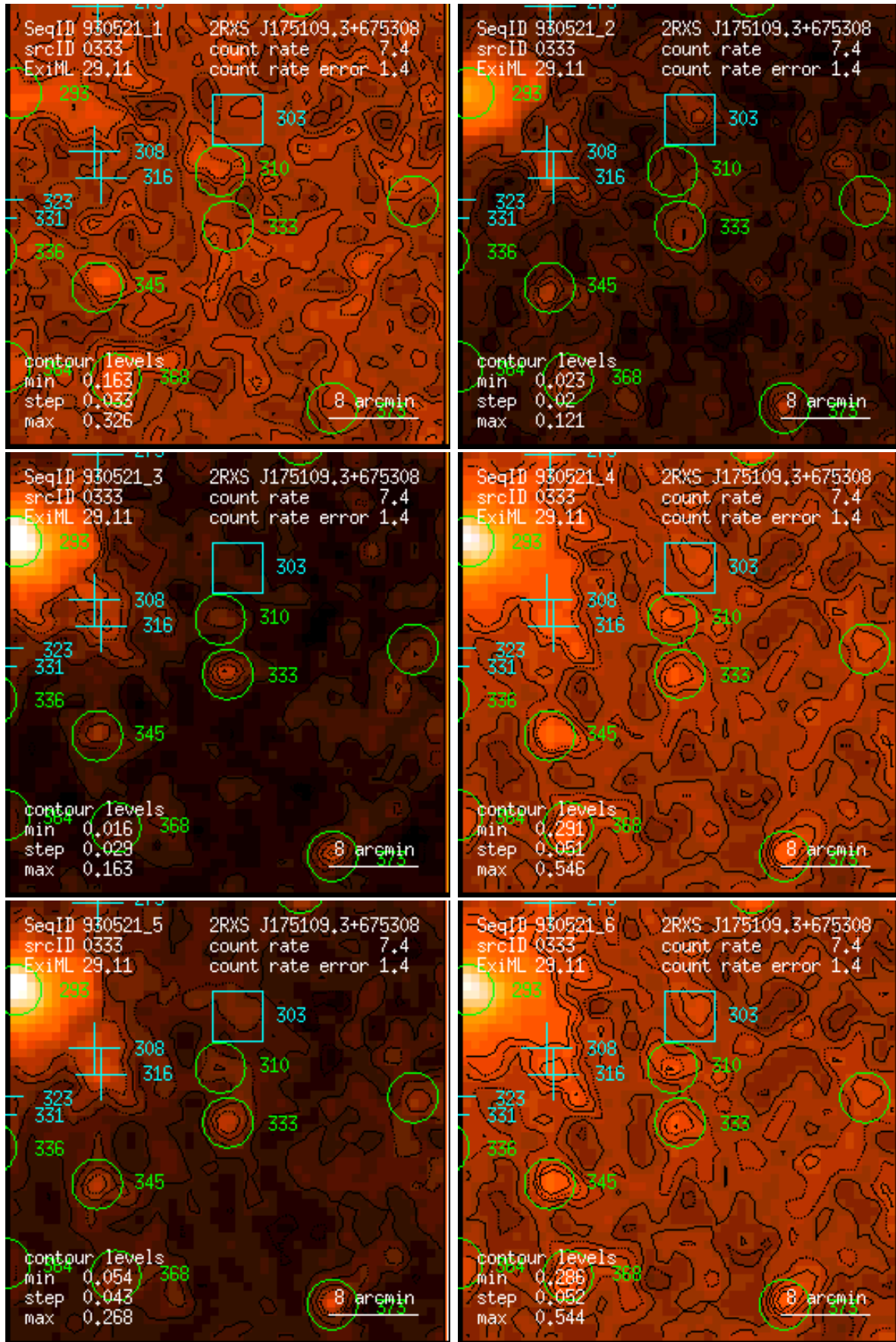
Figure 333: RASS 930521: detection 0333: band rate images, Gaussian filter: (1) PSPC channels 11 – 41, (2) 52 – 90, (3) 91 – 201, (4) 11 – 235, (5) 52 – 201, (6) 11 – 201. Broad band rates in counts/ks. Band rate contour levels in counts/ks/arcmin 2 .
