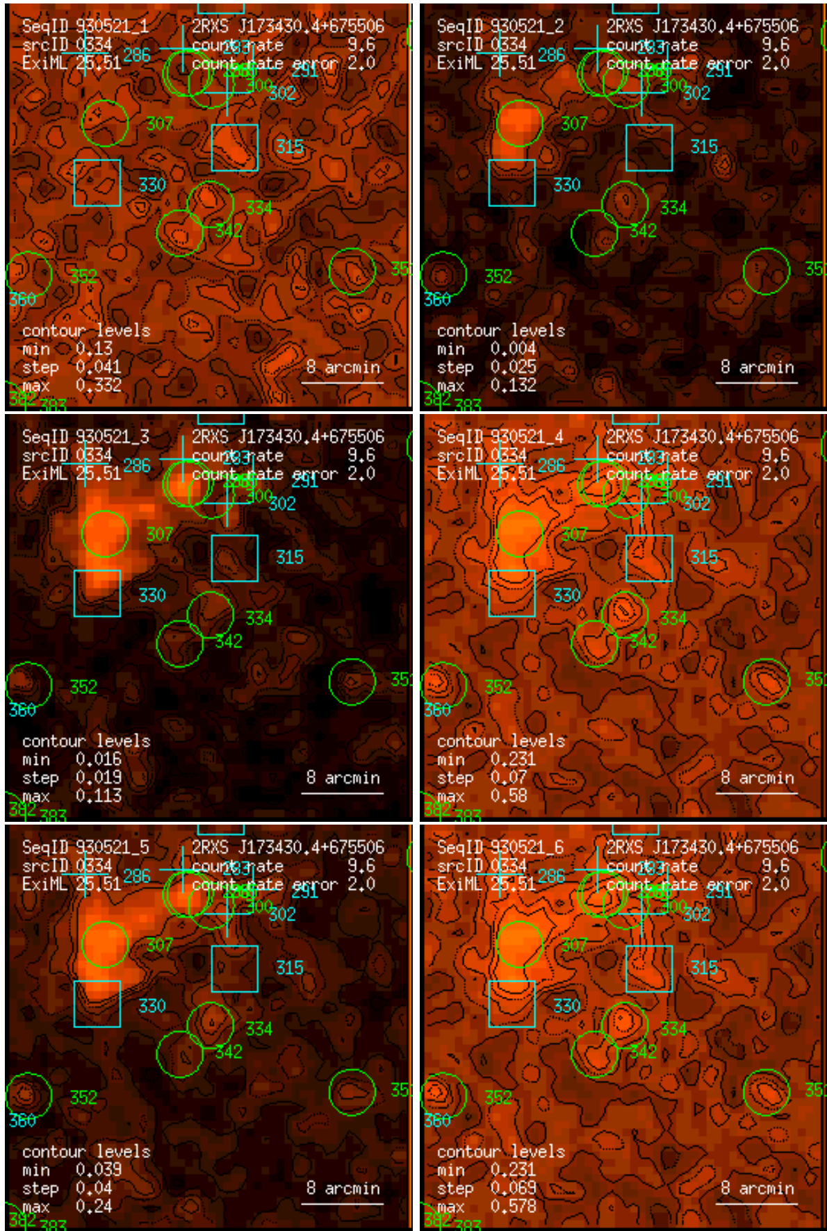
Figure 334: RASS 930521: detection 0334: band rate images, Gaussian filter: (1) PSPC channels 11 – 41, (2) 52 – 90, (3) 91 – 201, (4) 11 – 235, (5) 52 – 201, (6) 11 – 201. Broad band rates in counts/ks. Band rate contour levels in counts/ks/arcmin 2 .
