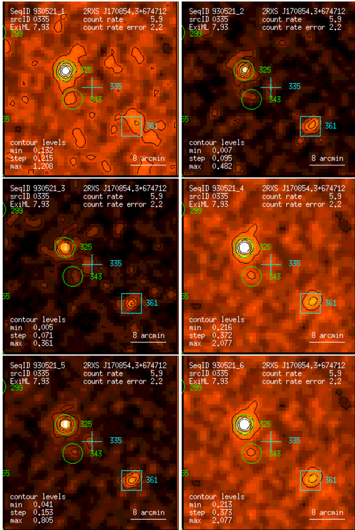
Figure 335: RASS 930521: detection 0335: band rate images, Gaussian filter: (1) PSPC channels 11 – 41, (2) 52 – 90, (3) 91 – 201, (4) 11 – 235, (5) 52 – 201, (6) 11 – 201. Broad band rates in counts/ks. Band rate contour levels in counts/ks/arcmin 2 .
