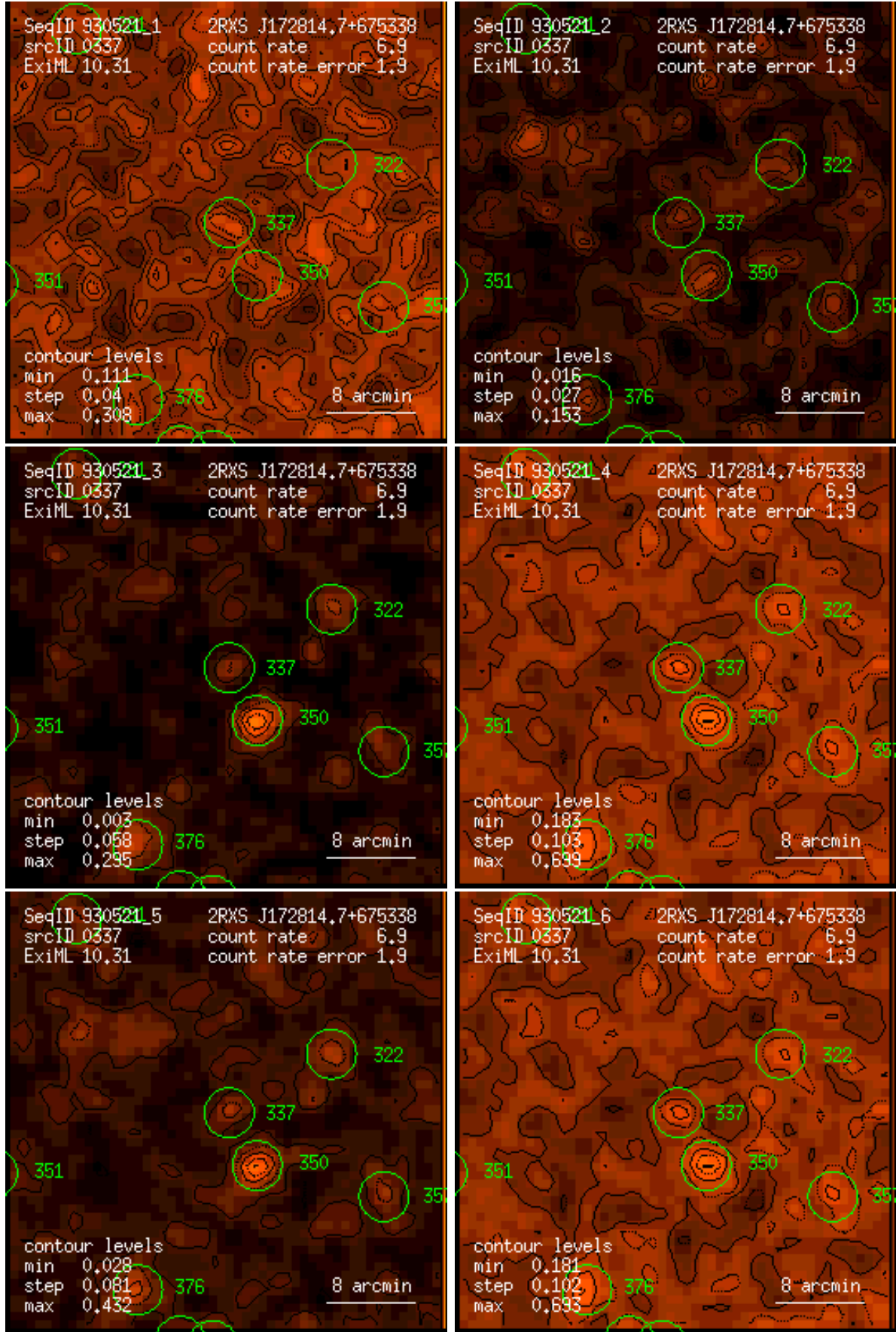
Figure 337: RASS 930521: detection 0337: band rate images, Gaussian filter: (1) PSPC channels 11 – 41, (2) 52 – 90, (3) 91 – 201, (4) 11 – 235, (5) 52 – 201, (6) 11 – 201. Broad band rates in counts/ks. Band rate contour levels in counts/ks/arcmin 2 .
