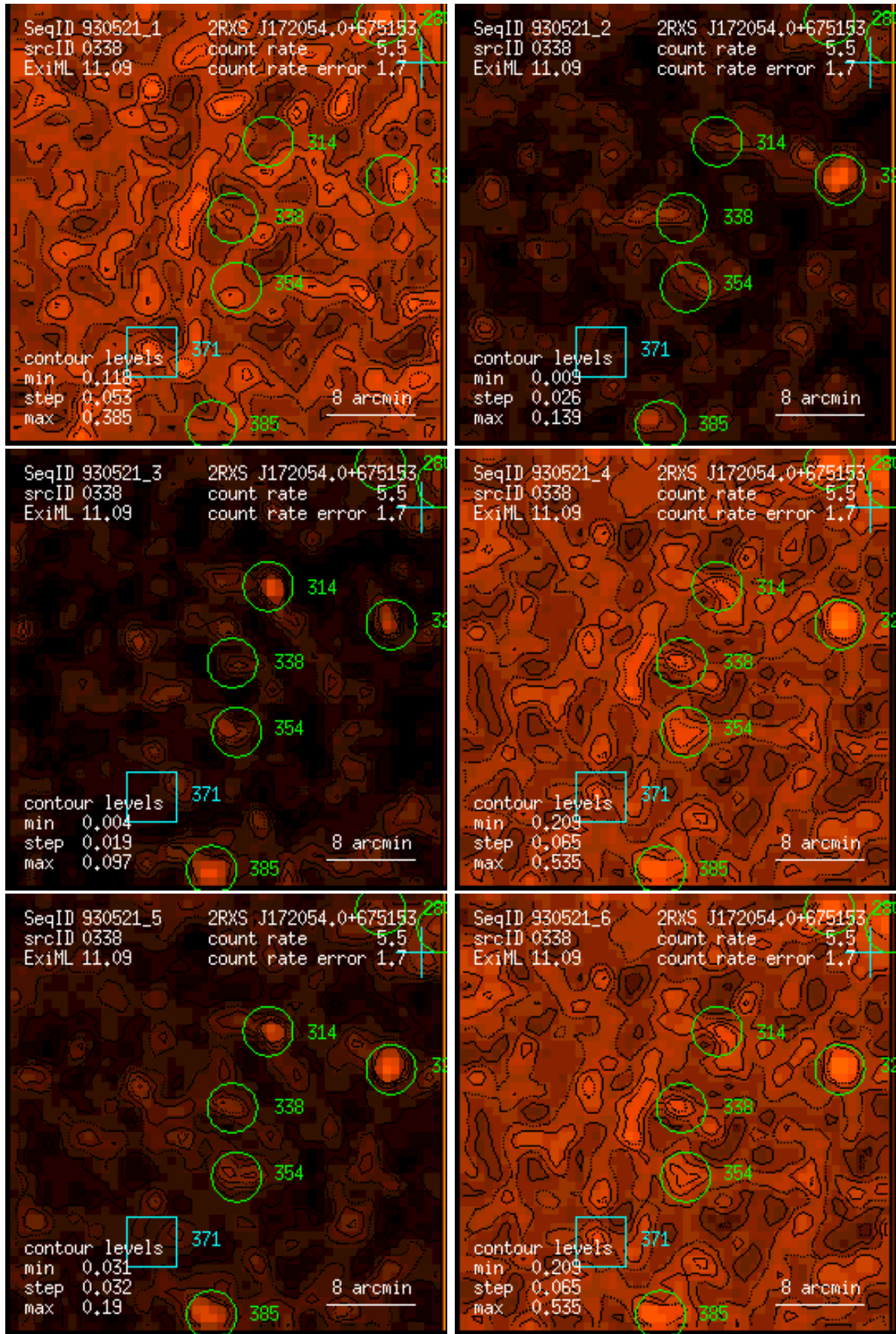
Figure 338: RASS 930521: detection 0338: band rate images, Gaussian filter: (1) PSPC channels 11 – 41, (2) 52 – 90, (3) 91 – 201, (4) 11 – 235, (5) 52 – 201, (6) 11 – 201. Broad band rates in counts/ks. Band rate contour levels in counts/ks/arcmin 2 .
