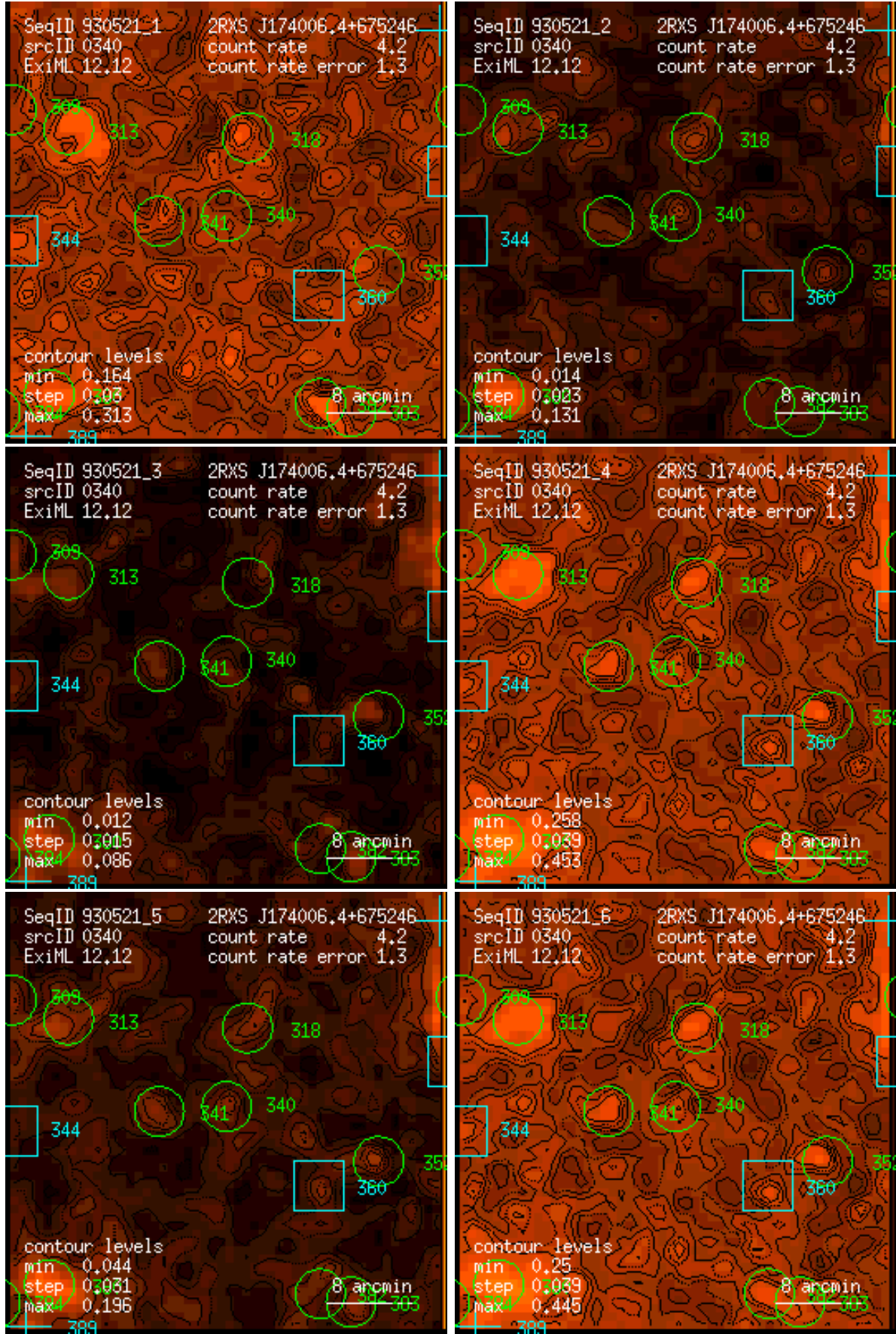
Figure 340: RASS 930521: detection 0340: band rate images, Gaussian filter: (1) PSPC channels 11 – 41, (2) 52 – 90, (3) 91 – 201, (4) 11 – 235, (5) 52 – 201, (6) 11 – 201. Broad band rates in counts/ks. Band rate contour levels in counts/ks/arcmin 2 .
