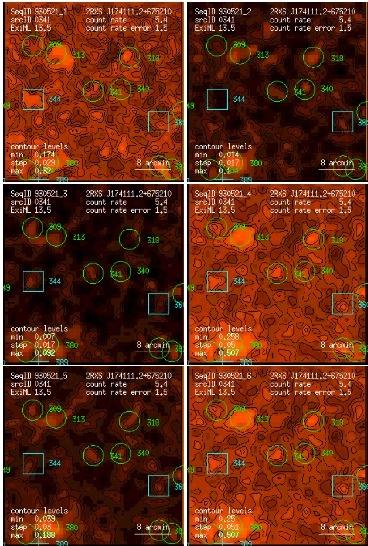
Figure 341: RASS 930521: detection 0341: band rate images, Gaussian filter: (1) PSPC channels 11 – 41, (2) 52 – 90, (3) 91 – 201, (4) 11 – 235, (5) 52 – 201, (6) 11 – 201. Broad band rates in counts/ks. Band rate contour levels in counts/ks/arcmin 2 .
