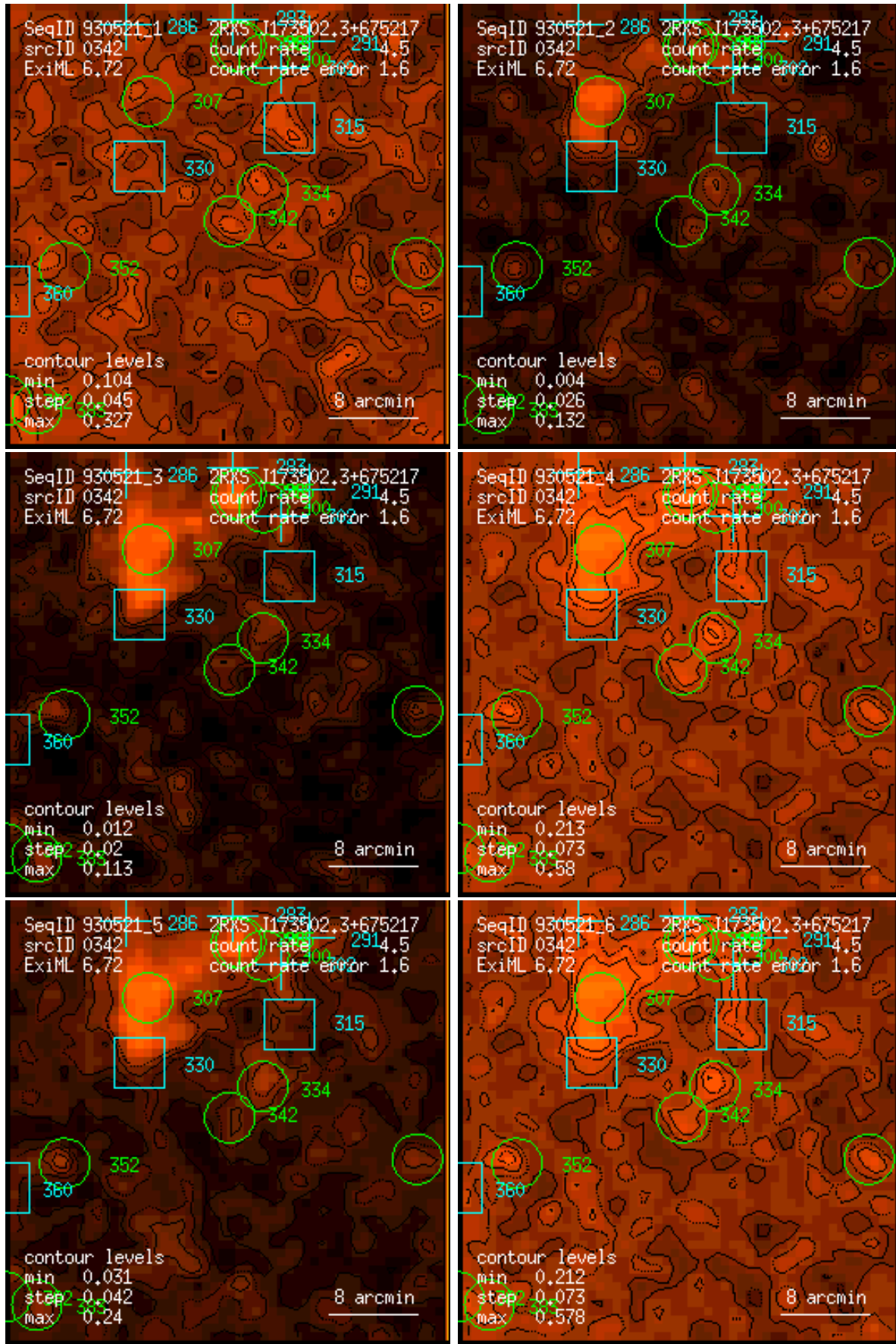
Figure 342: RASS 930521: detection 0342: band rate images, Gaussian filter: (1) PSPC channels 11 – 41, (2) 52 – 90, (3) 91 – 201, (4) 11 – 235, (5) 52 – 201, (6) 11 – 201. Broad band rates in counts/ks. Band rate contour levels in counts/ks/arcmin 2 .
