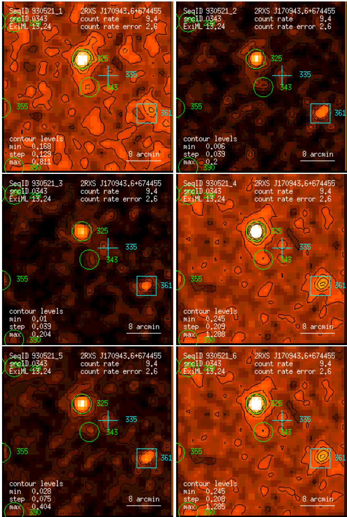
Figure 343: RASS 930521: detection 0343: band rate images, Gaussian filter: (1) PSPC channels 11 – 41, (2) 52 – 90, (3) 91 – 201, (4) 11 – 235, (5) 52 – 201, (6) 11 – 201. Broad band rates in counts/ks. Band rate contour levels in counts/ks/arcmin 2 .
