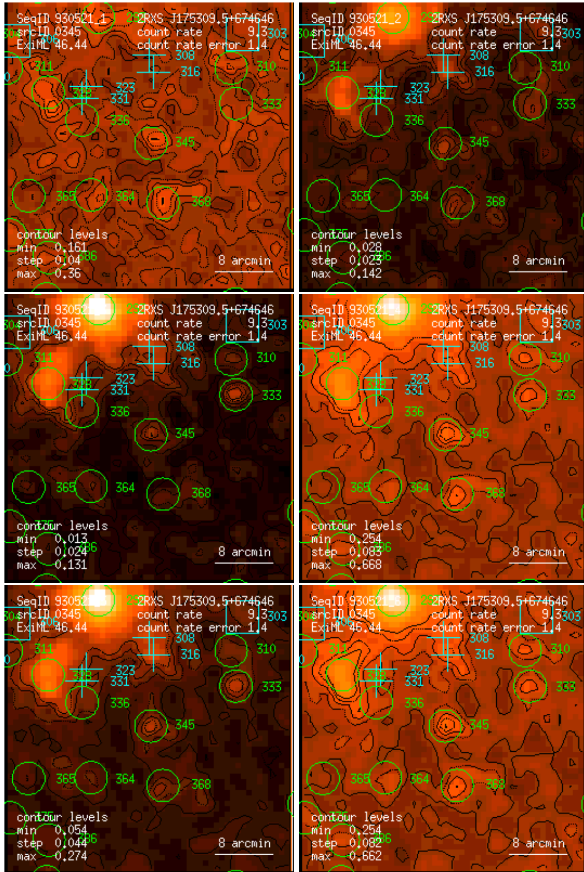
Figure 345: RASS 930521: detection 0345: band rate images, Gaussian filter: (1) PSPC channels 11 – 41, (2) 52 – 90, (3) 91 – 201, (4) 11 – 235, (5) 52 – 201, (6) 11 – 201. Broad band rates in counts/ks. Band rate contour levels in counts/ks/arcmin 2 .
