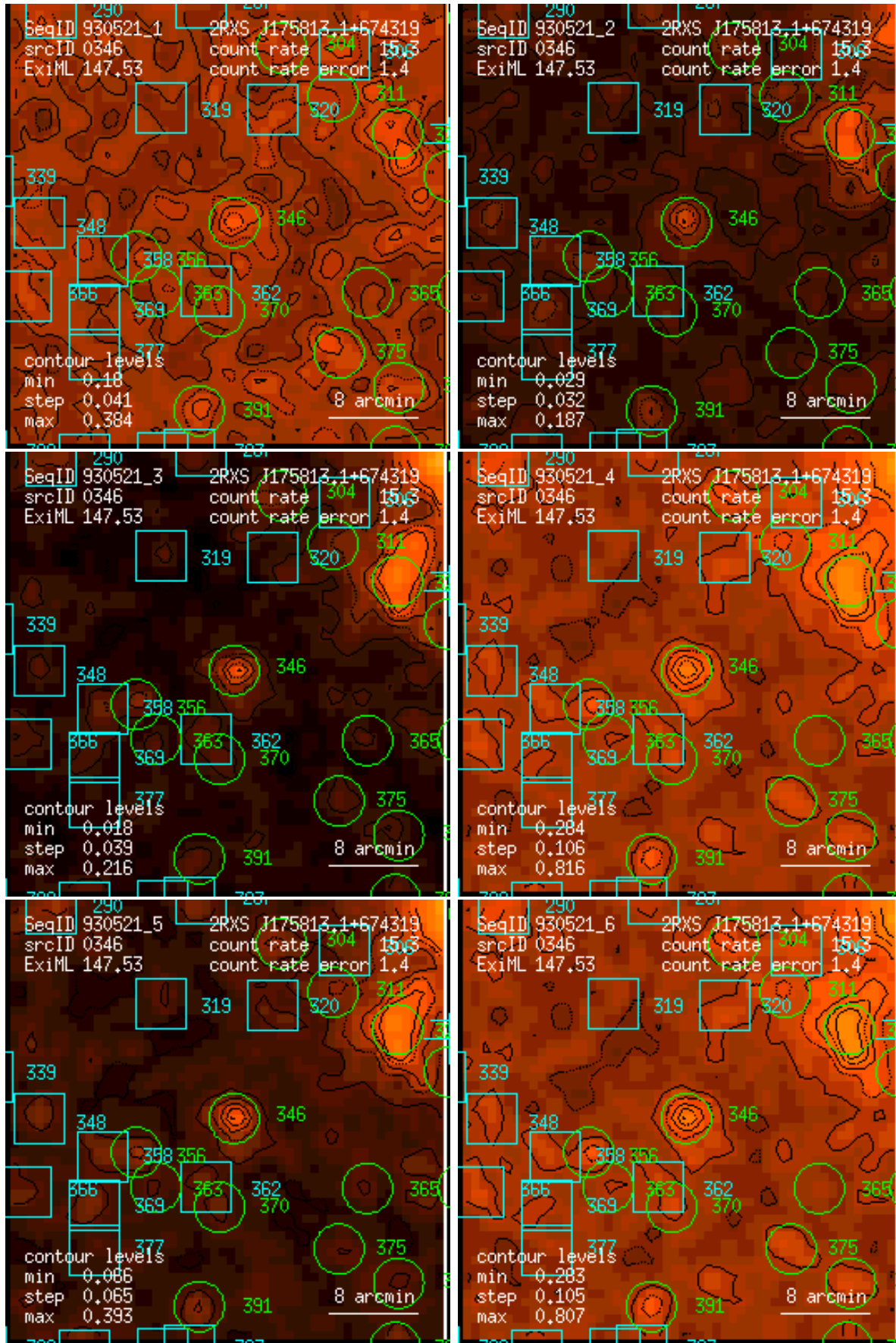
Figure 346: RASS 930521: detection 0346: band rate images, Gaussian filter: (1) PSPC channels 11 – 41, (2) 52 – 90, (3) 91 – 201, (4) 11 – 235, (5) 52 – 201, (6) 11 – 201. Broad band rates in counts/ks. Band rate contour levels in counts/ks/arcmin 2 .
