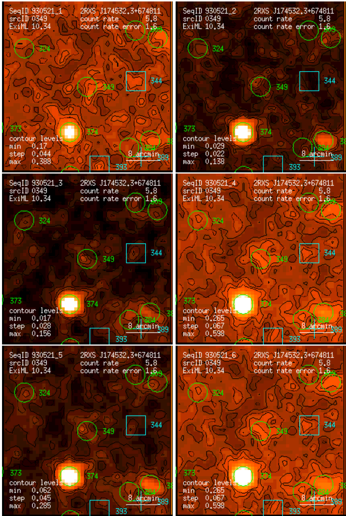
Figure 349: RASS 930521: detection 0349: band rate images, Gaussian filter: (1) PSPC channels 11 – 41, (2) 52 – 90, (3) 91 – 201, (4) 11 – 235, (5) 52 – 201, (6) 11 – 201. Broad band rates in counts/ks. Band rate contour levels in counts/ks/arcmin 2 .
