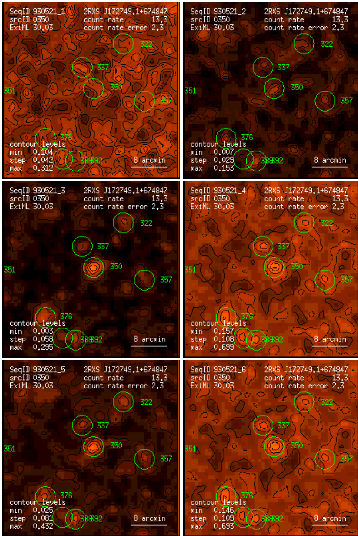
Figure 350: RASS 930521: detection 0350: band rate images, Gaussian filter: (1) PSPC channels 11 – 41, (2) 52 – 90, (3) 91 – 201, (4) 11 – 235, (5) 52 – 201, (6) 11 – 201. Broad band rates in counts/ks. Band rate contour levels in counts/ks/arcmin 2 .
