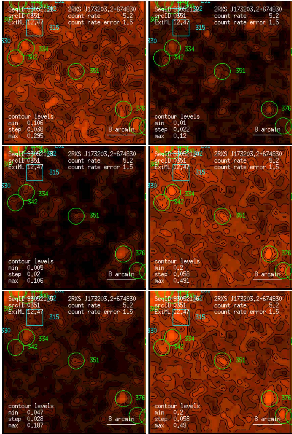
Figure 351: RASS 930521: detection 0351: band rate images, Gaussian filter: (1) PSPC channels 11 – 41, (2) 52 – 90, (3) 91 – 201, (4) 11 – 235, (5) 52 – 201, (6) 11 – 201. Broad band rates in counts/ks. Band rate contour levels in counts/ks/arcmin 2 .
