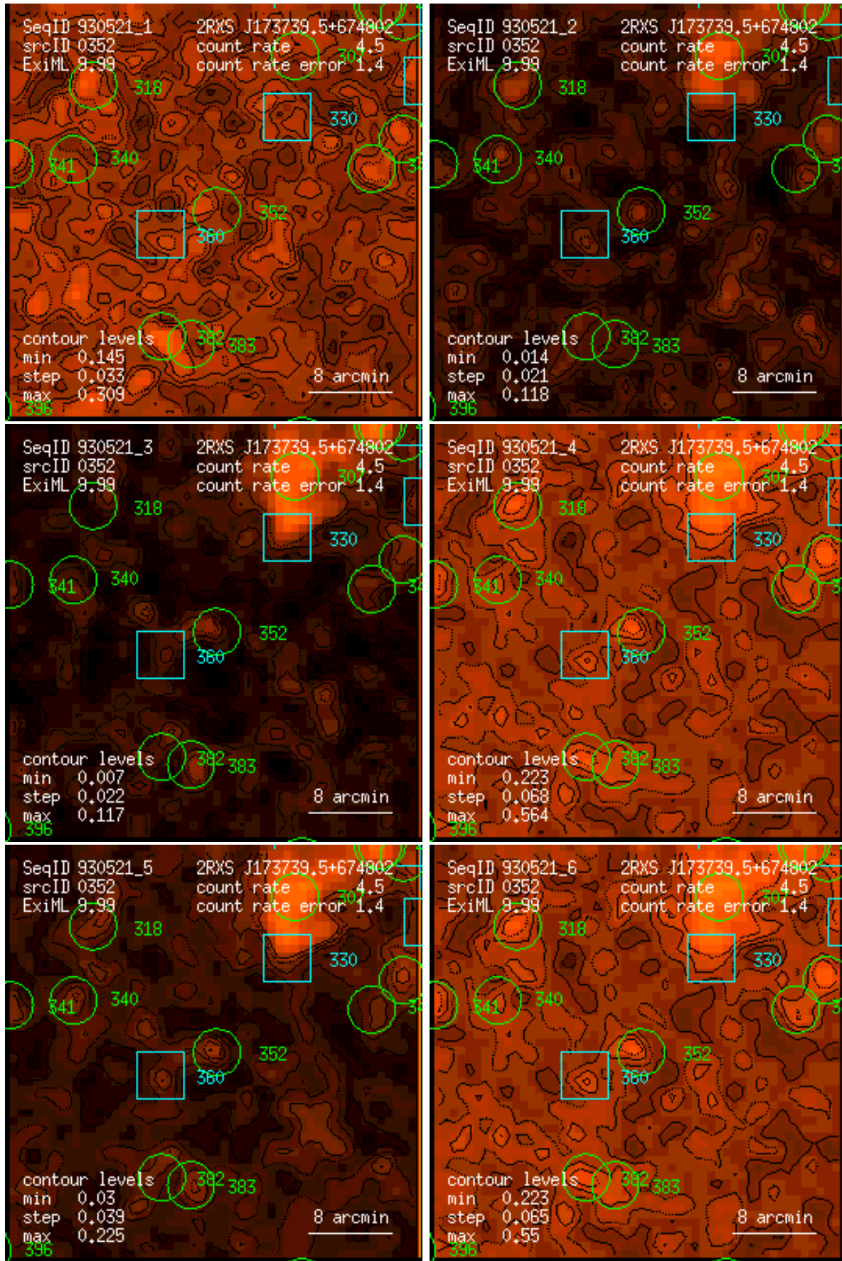
Figure 352: RASS 930521: detection 0352: band rate images, Gaussian filter: (1) PSPC channels 11 – 41, (2) 52 – 90, (3) 91 – 201, (4) 11 – 235, (5) 52 – 201, (6) 11 – 201. Broad band rates in counts/ks. Band rate contour levels in counts/ks/arcmin 2 .
