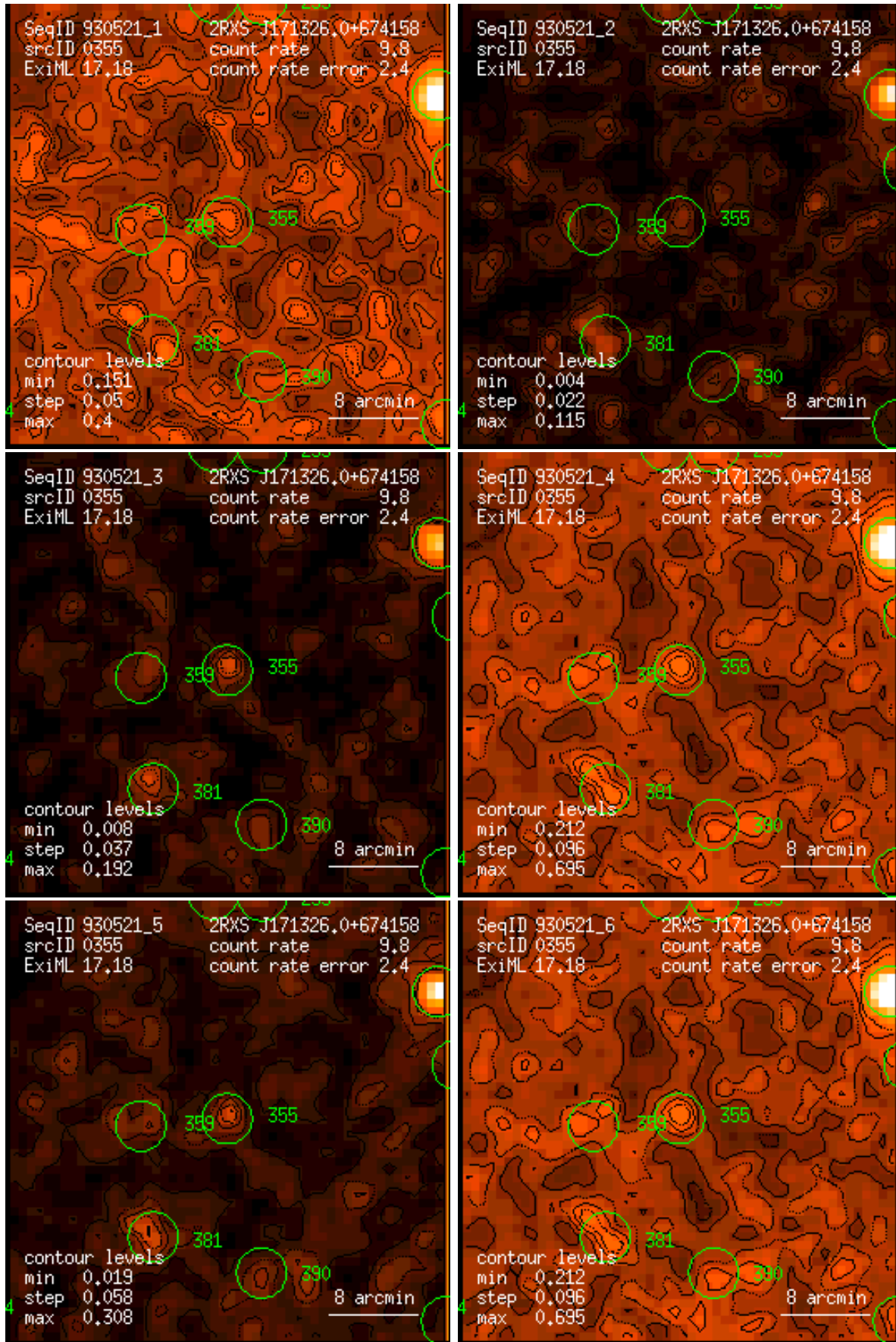
Figure 355: RASS 930521: detection 0355: band rate images, Gaussian filter: (1) PSPC channels 11 – 41, (2) 52 – 90, (3) 91 – 201, (4) 11 – 235, (5) 52 – 201, (6) 11 – 201. Broad band rates in counts/ks. Band rate contour levels in counts/ks/arcmin 2 .
