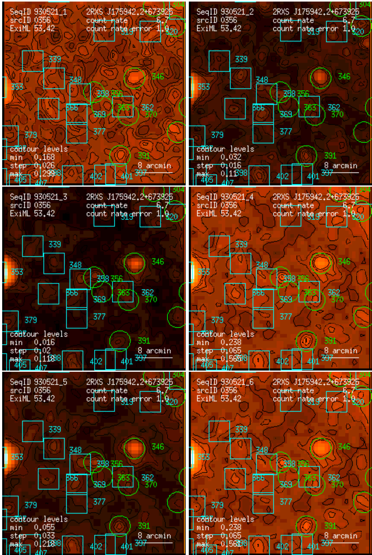
Figure 356: RASS 930521: detection 0356: band rate images, Gaussian filter: (1) PSPC channels 11 – 41, (2) 52 – 90, (3) 91 – 201, (4) 11 – 235, (5) 52 – 201, (6) 11 – 201. Broad band rates in counts/ks. Band rate contour levels in counts/ks/arcmin 2 .
