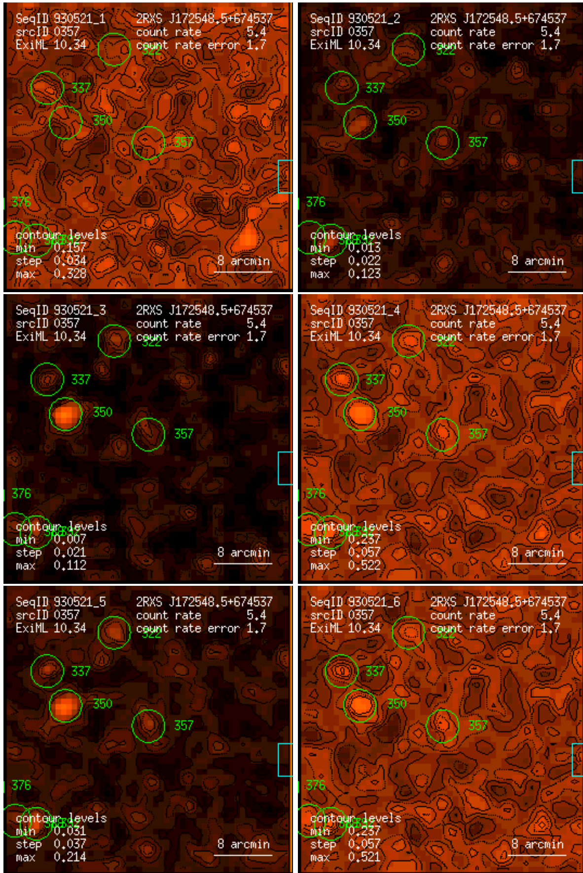
Figure 357: RASS 930521: detection 0357: band rate images, Gaussian filter: (1) PSPC channels 11 – 41, (2) 52 – 90, (3) 91 – 201, (4) 11 – 235, (5) 52 – 201, (6) 11 – 201. Broad band rates in counts/ks. Band rate contour levels in counts/ks/arcmin 2 .
