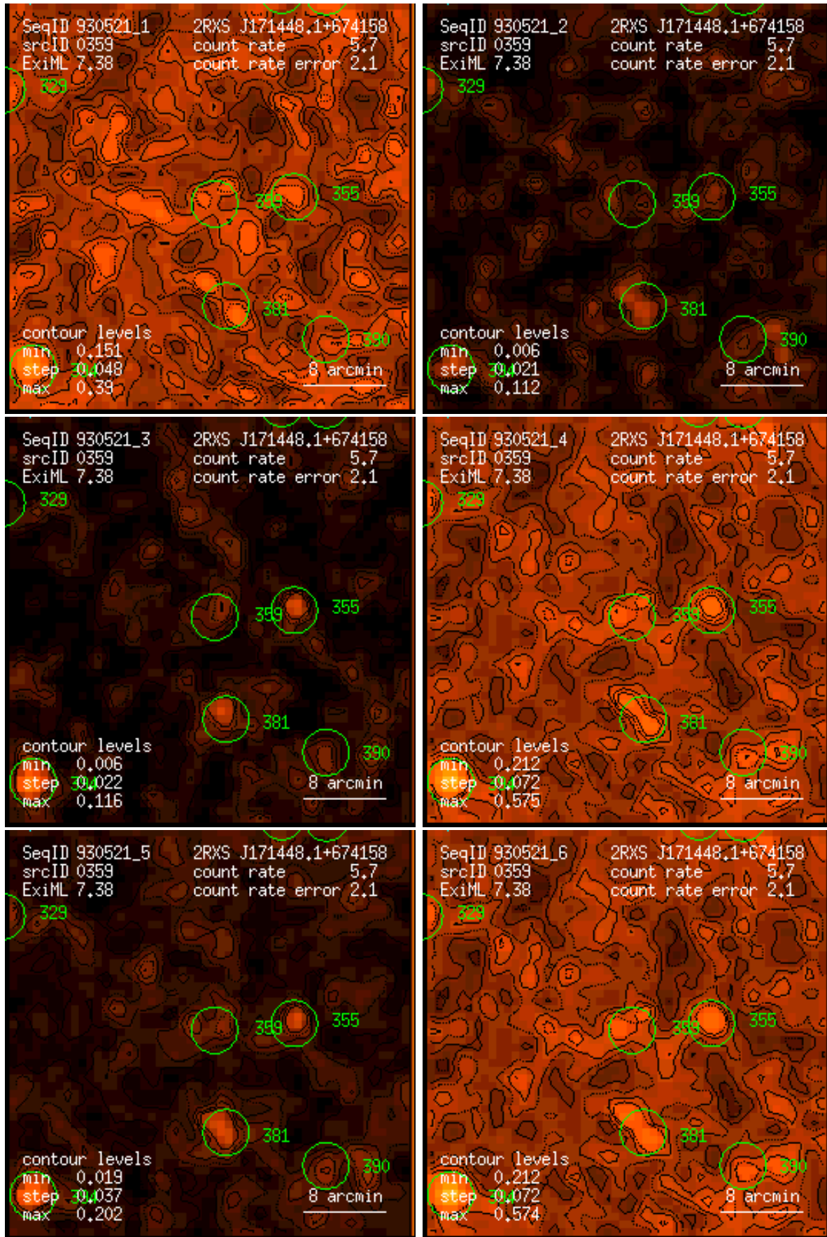
Figure 359: RASS 930521: detection 0359: band rate images, Gaussian filter: (1) PSPC channels 11 – 41, (2) 52 – 90, (3) 91 – 201, (4) 11 – 235, (5) 52 – 201, (6) 11 – 201. Broad band rates in counts/ks. Band rate contour levels in counts/ks/arcmin 2 .
