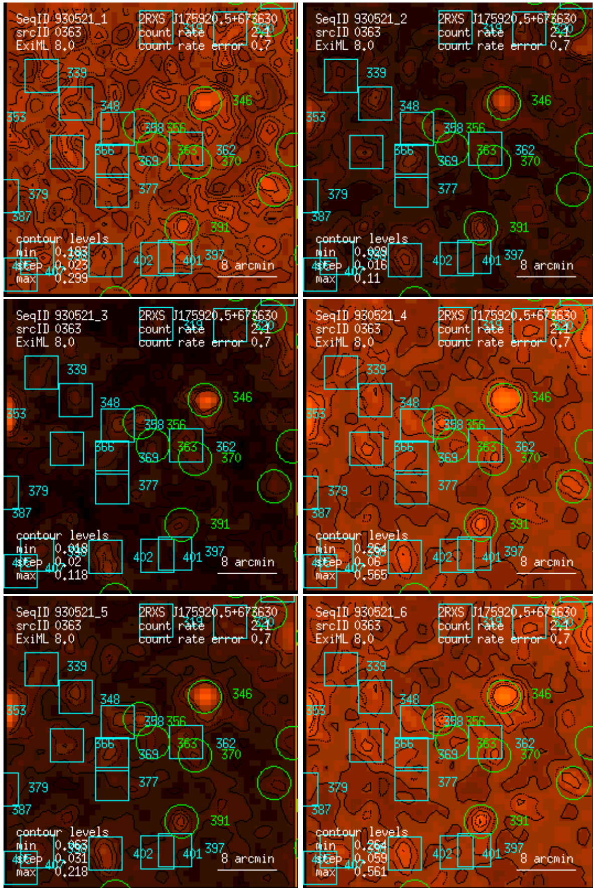
Figure 363: RASS 930521: detection 0363: band rate images, Gaussian filter: (1) PSPC channels 11 – 41, (2) 52 – 90, (3) 91 – 201, (4) 11 – 235, (5) 52 – 201, (6) 11 – 201. Broad band rates in counts/ks. Band rate contour levels in counts/ks/arcmin 2 .
