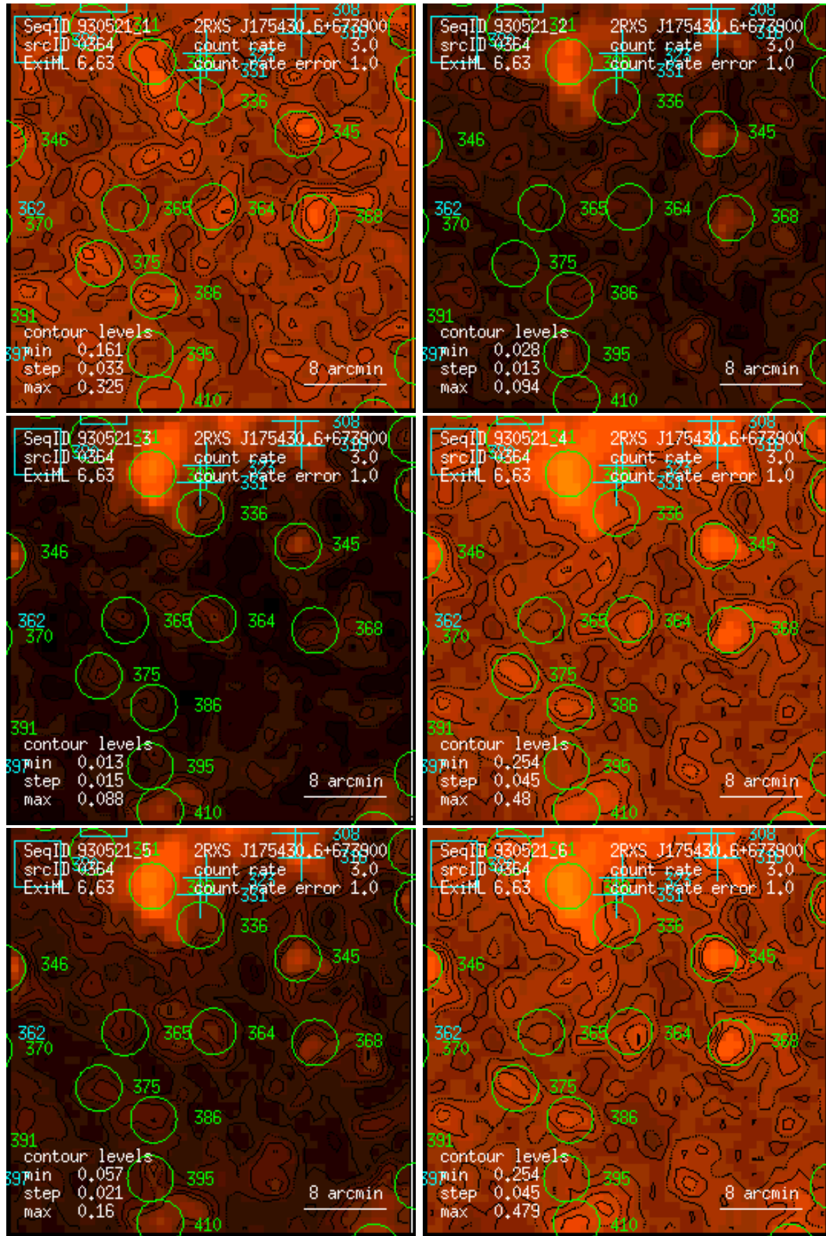
Figure 364: RASS 930521: detection 0364: band rate images, Gaussian filter: (1) PSPC channels 11 – 41, (2) 52 – 90, (3) 91 – 201, (4) 11 – 235, (5) 52 – 201, (6) 11 – 201. Broad band rates in counts/ks. Band rate contour levels in counts/ks/arcmin 2 .
