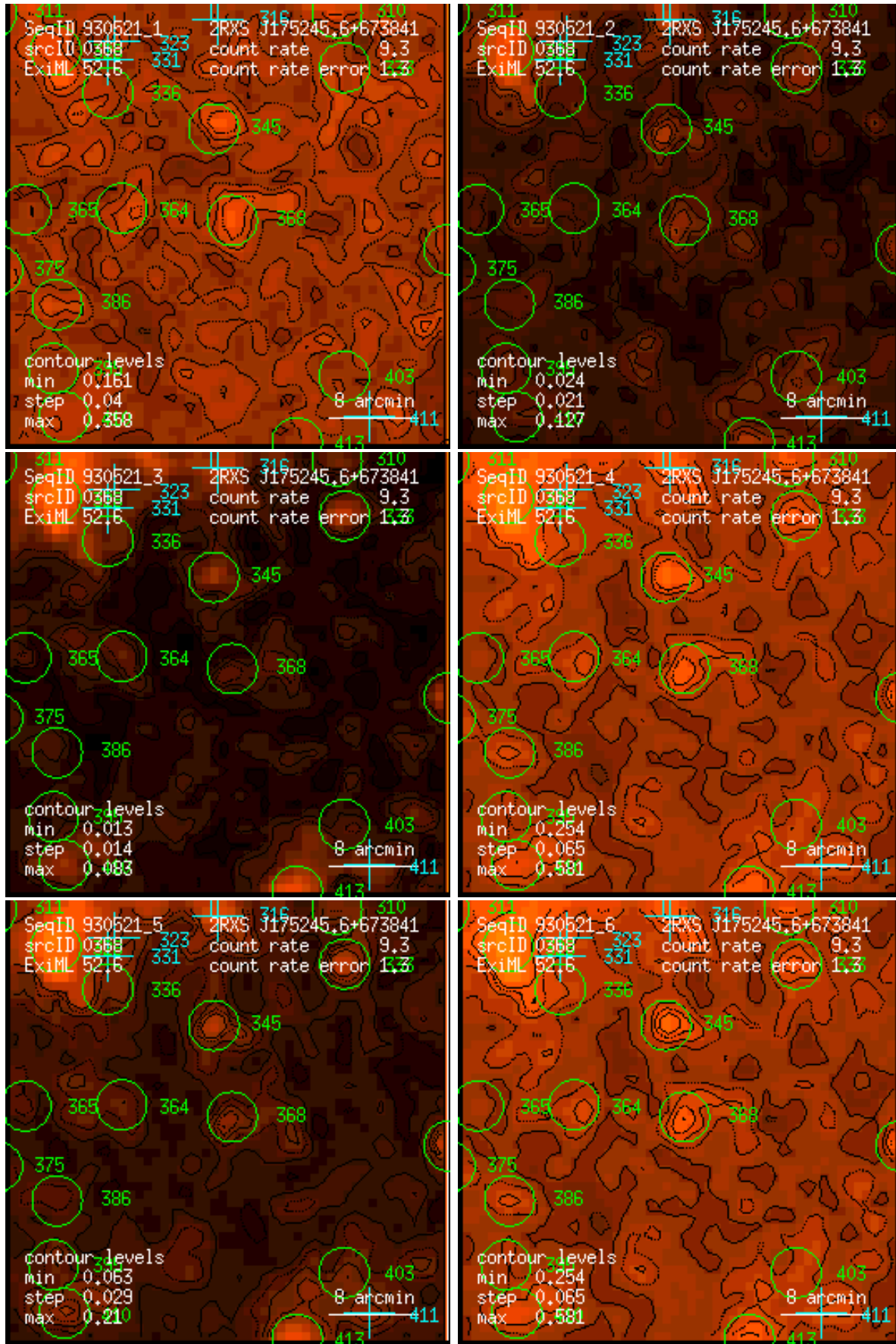
Figure 368: RASS 930521: detection 0368: band rate images, Gaussian filter: (1) PSPC channels 11 – 41, (2) 52 – 90, (3) 91 – 201, (4) 11 – 235, (5) 52 – 201, (6) 11 – 201. Broad band rates in counts/ks. Band rate contour levels in counts/ks/arcmin 2 .
