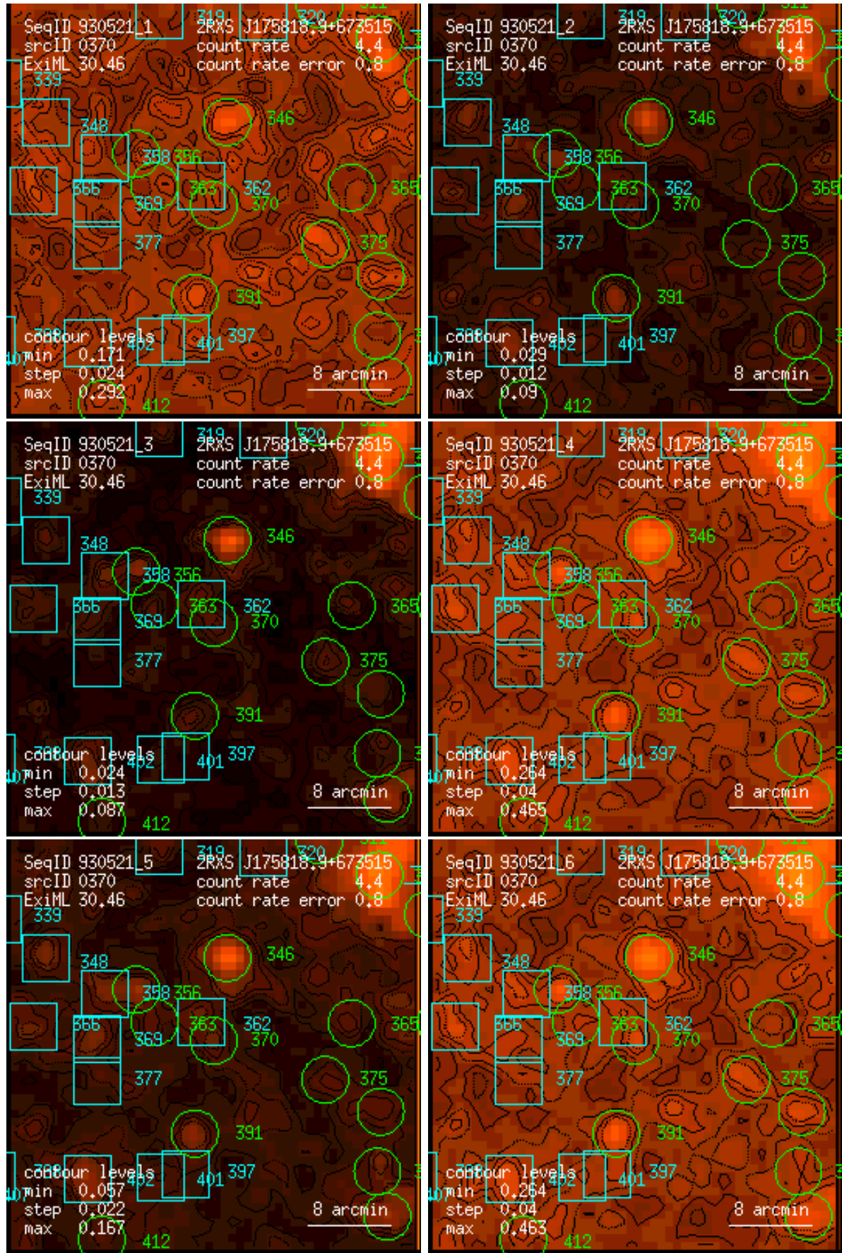
Figure 370: RASS 930521: detection 0370: band rate images, Gaussian filter: (1) PSPC channels 11 – 41, (2) 52 – 90, (3) 91 – 201, (4) 11 – 235, (5) 52 – 201, (6) 11 – 201. Broad band rates in counts/ks. Band rate contour levels in counts/ks/arcmin 2 .
