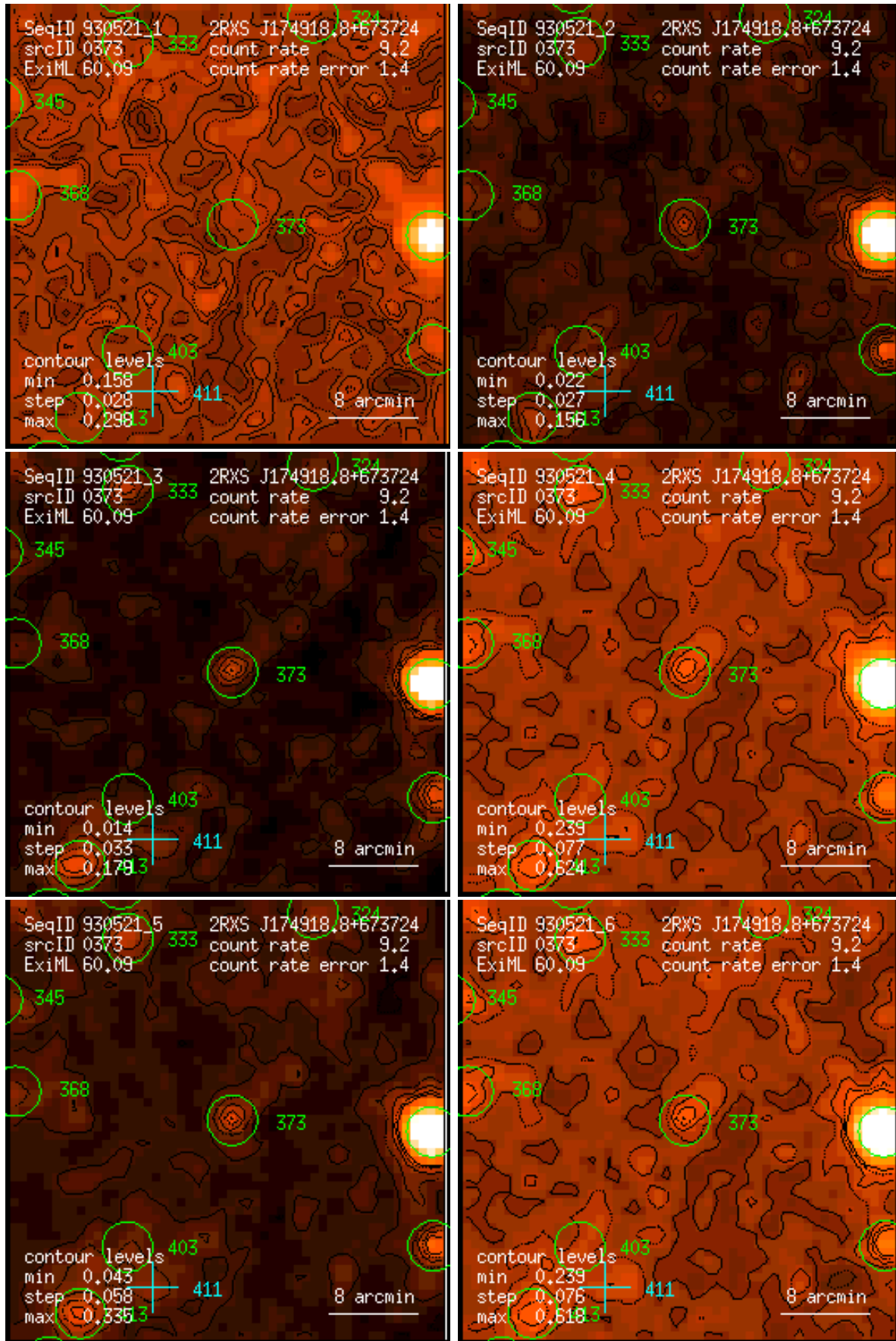
Figure 373: RASS 930521: detection 0373: band rate images, Gaussian filter: (1) PSPC channels 11 – 41, (2) 52 – 90, (3) 91 – 201, (4) 11 – 235, (5) 52 – 201, (6) 11 – 201. Broad band rates in counts/ks. Band rate contour levels in counts/ks/arcmin 2 .
