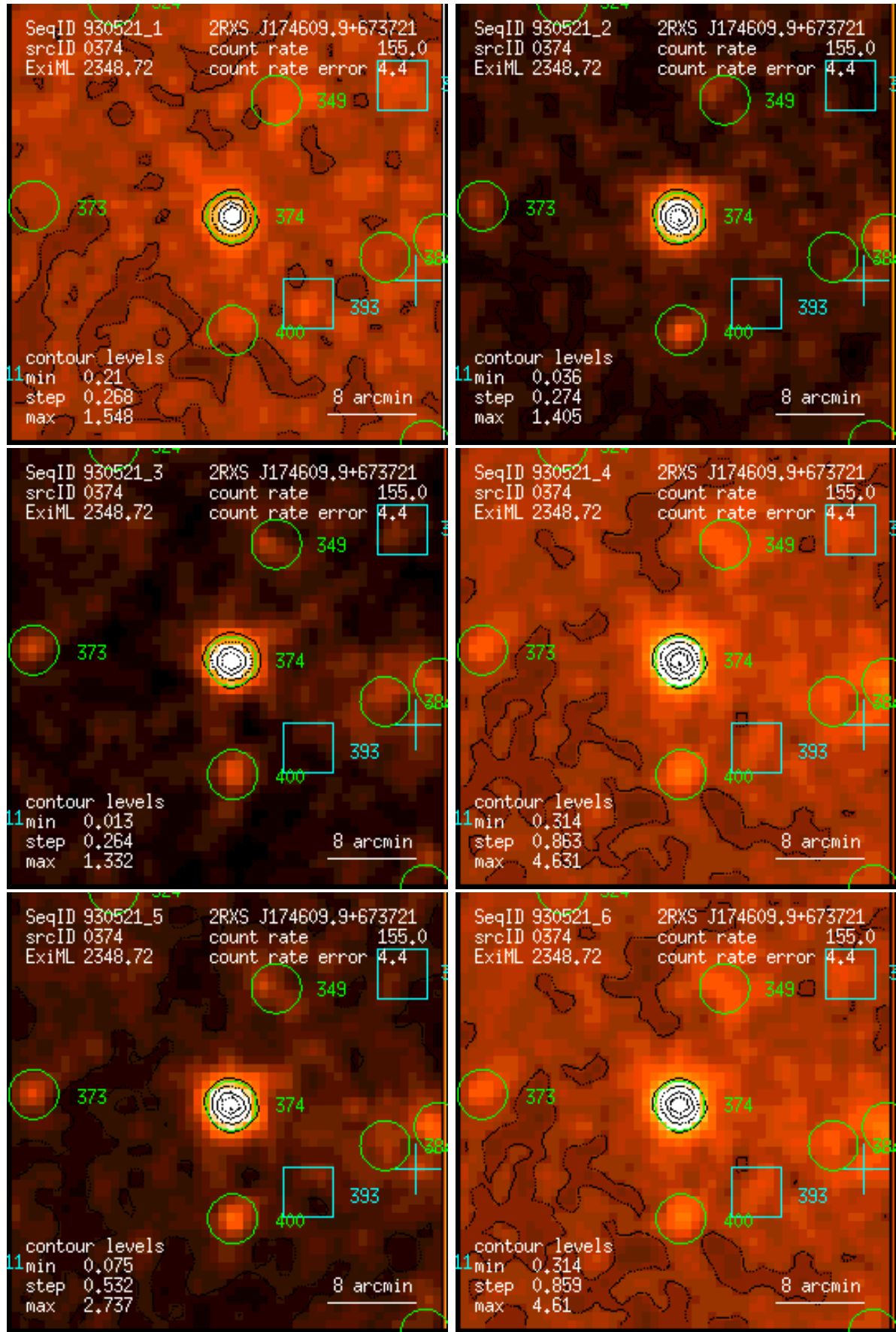
Figure 374: RASS 930521: detection 0374: band rate images, Gaussian filter: (1) PSPC channels 11 – 41, (2) 52 – 90, (3) 91 – 201, (4) 11 – 235, (5) 52 – 201, (6) 11 – 201. Broad band rates in counts/ks. Band rate contour levels in counts/ks/arcmin 2 .
