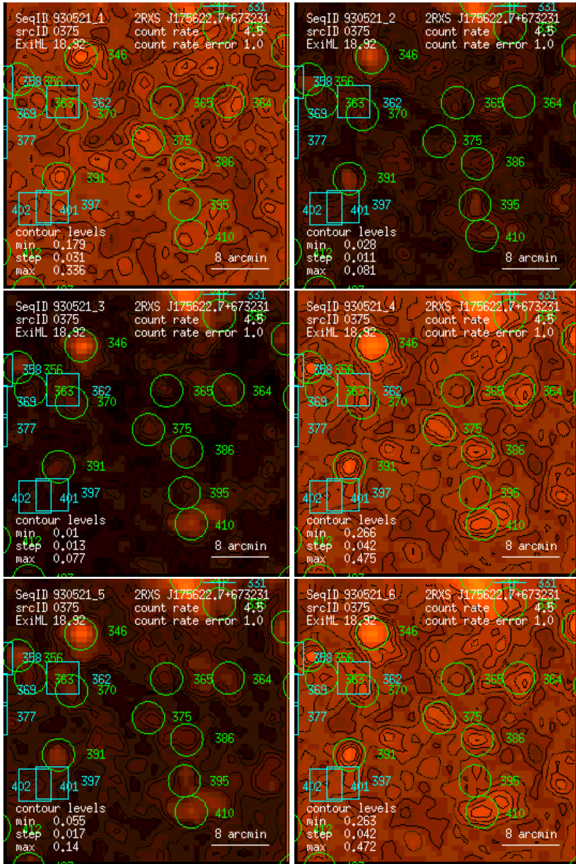
Figure 375: RASS 930521: detection 0375: band rate images, Gaussian filter: (1) PSPC channels 11 – 41, (2) 52 – 90, (3) 91 – 201, (4) 11 – 235, (5) 52 – 201, (6) 11 – 201. Broad band rates in counts/ks. Band rate contour levels in counts/ks/arcmin 2 .
