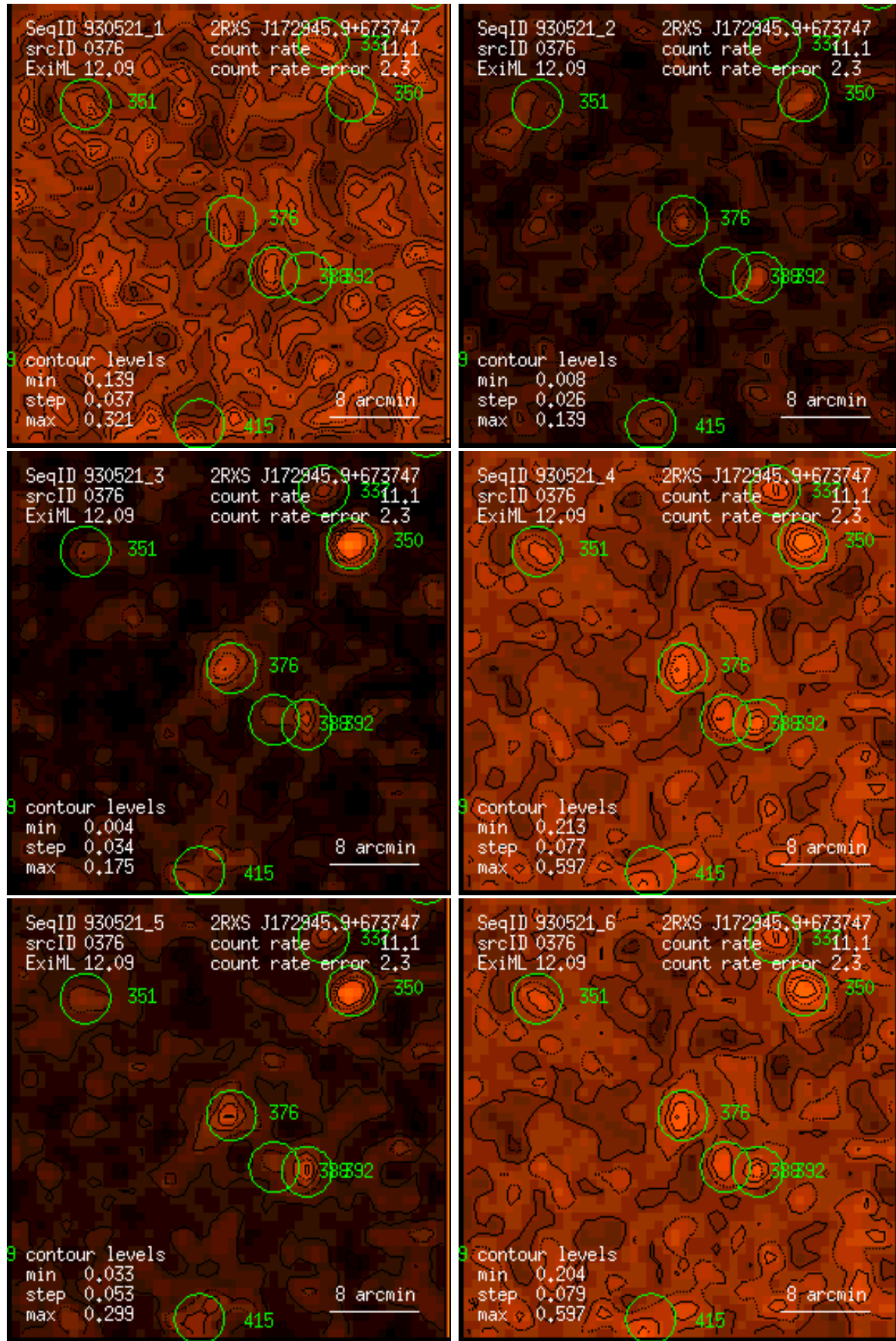
Figure 376: RASS 930521: detection 0376: band rate images, Gaussian filter: (1) PSPC channels 11 – 41, (2) 52 – 90, (3) 91 – 201, (4) 11 – 235, (5) 52 – 201, (6) 11 – 201. Broad band rates in counts/ks. Band rate contour levels in counts/ks/arcmin 2 .
