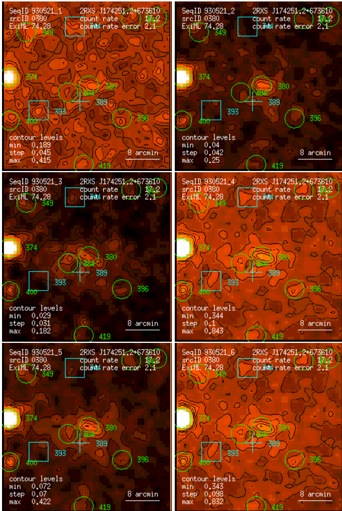
Figure 380: RASS 930521: detection 0380: band rate images, Gaussian filter: (1) PSPC channels 11 – 41, (2) 52 – 90, (3) 91 – 201, (4) 11 – 235, (5) 52 – 201, (6) 11 – 201. Broad band rates in counts/ks. Band rate contour levels in counts/ks/arcmin 2 .
