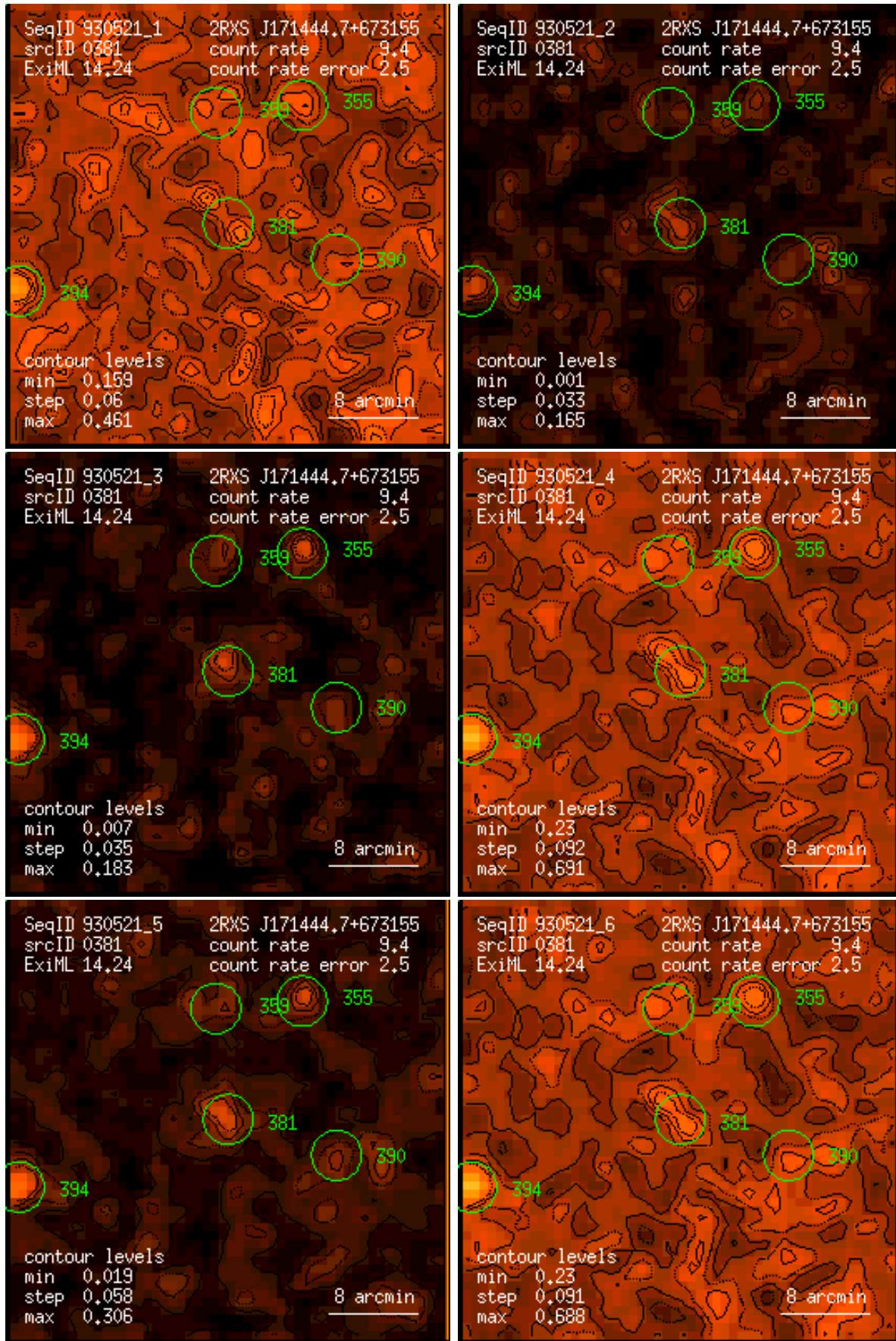
Figure 381: RASS 930521: detection 0381: band rate images, Gaussian filter: (1) PSPC channels 11 – 41, (2) 52 – 90, (3) 91 – 201, (4) 11 – 235, (5) 52 – 201, (6) 11 – 201. Broad band rates in counts/ks. Band rate contour levels in counts/ks/arcmin 2 .
