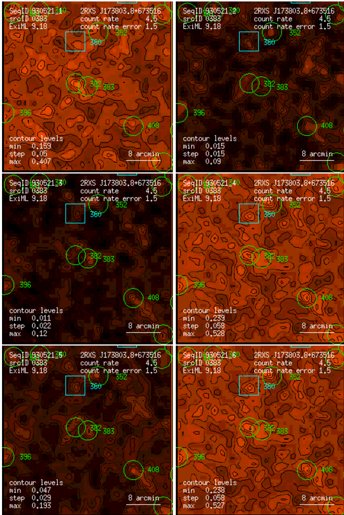
Figure 383: RASS 930521: detection 0383: band rate images, Gaussian filter: (1) PSPC channels 11 – 41, (2) 52 – 90, (3) 91 – 201, (4) 11 – 235, (5) 52 – 201, (6) 11 – 201. Broad band rates in counts/ks. Band rate contour levels in counts/ks/arcmin 2 .
