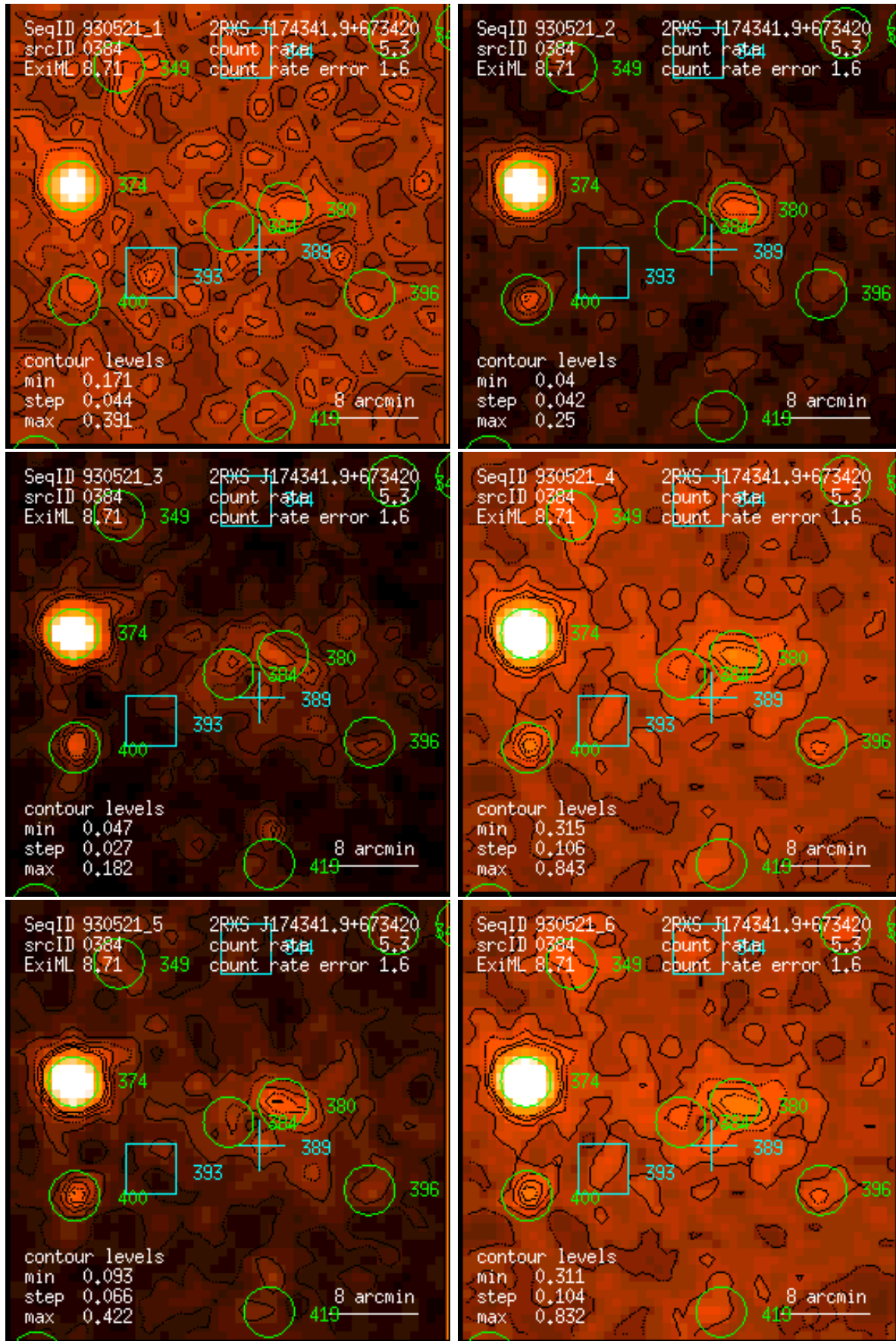
Figure 384: RASS 930521: detection 0384: band rate images, Gaussian filter: (1) PSPC channels 11 – 41, (2) 52 – 90, (3) 91 – 201, (4) 11 – 235, (5) 52 – 201, (6) 11 – 201. Broad band rates in counts/ks. Band rate contour levels in counts/ks/arcmin 2 .
