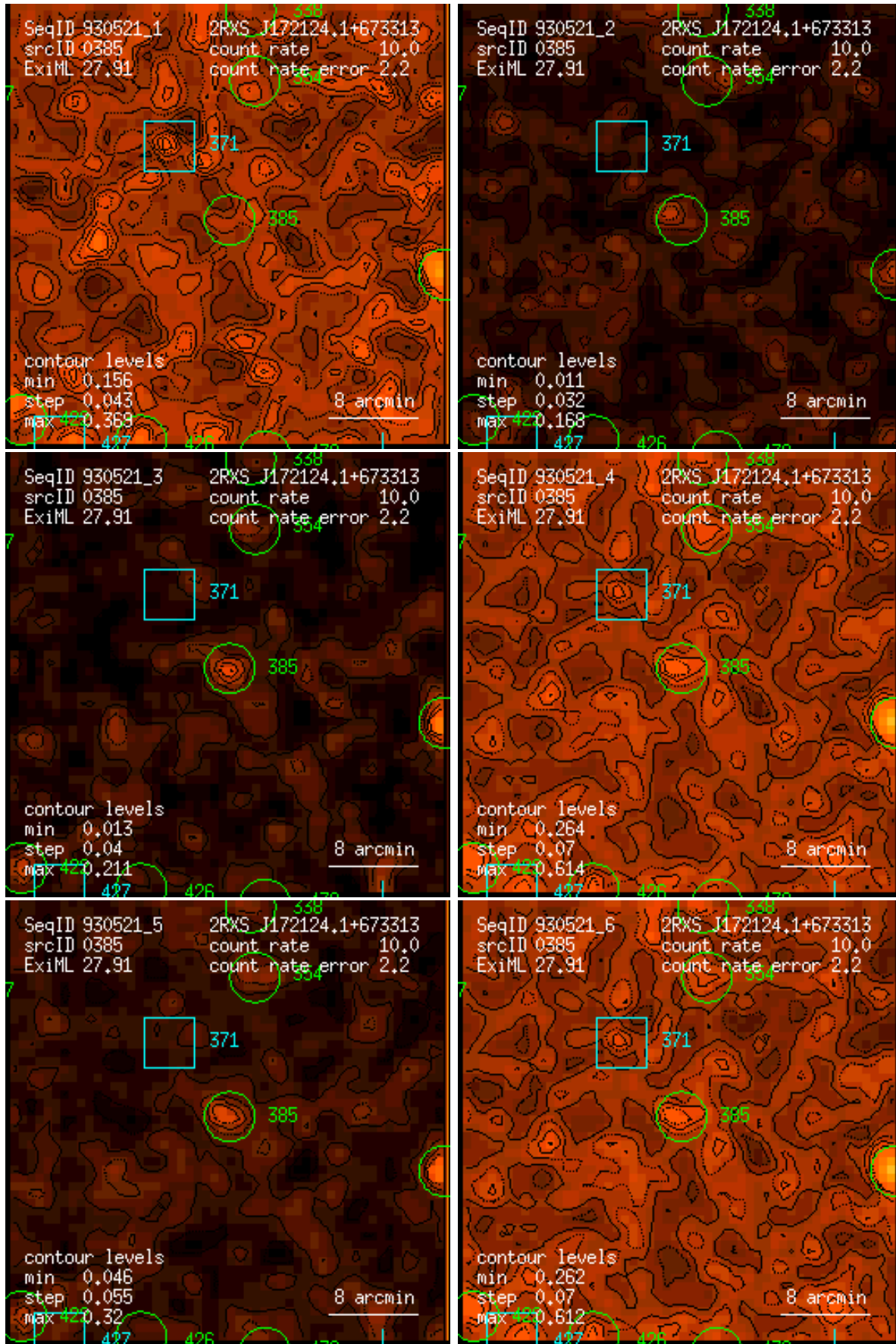
Figure 385: RASS 930521: detection 0385: band rate images, Gaussian filter: (1) PSPC channels 11 – 41, (2) 52 – 90, (3) 91 – 201, (4) 11 – 235, (5) 52 – 201, (6) 11 – 201. Broad band rates in counts/ks. Band rate contour levels in counts/ks/arcmin 2 .
