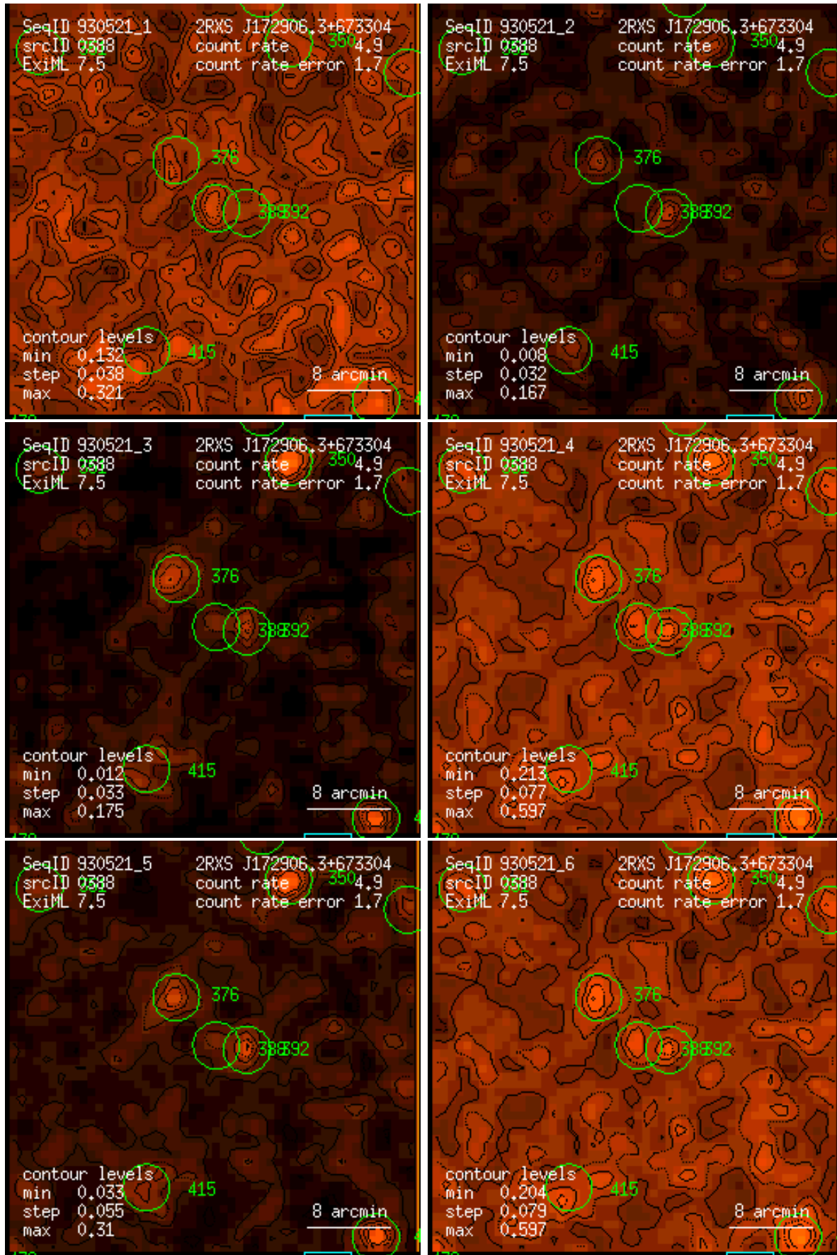
Figure 388: RASS 930521: detection 0388: band rate images, Gaussian filter: (1) PSPC channels 11 – 41, (2) 52 – 90, (3) 91 – 201, (4) 11 – 235, (5) 52 – 201, (6) 11 – 201. Broad band rates in counts/ks. Band rate contour levels in counts/ks/arcmin 2 .
