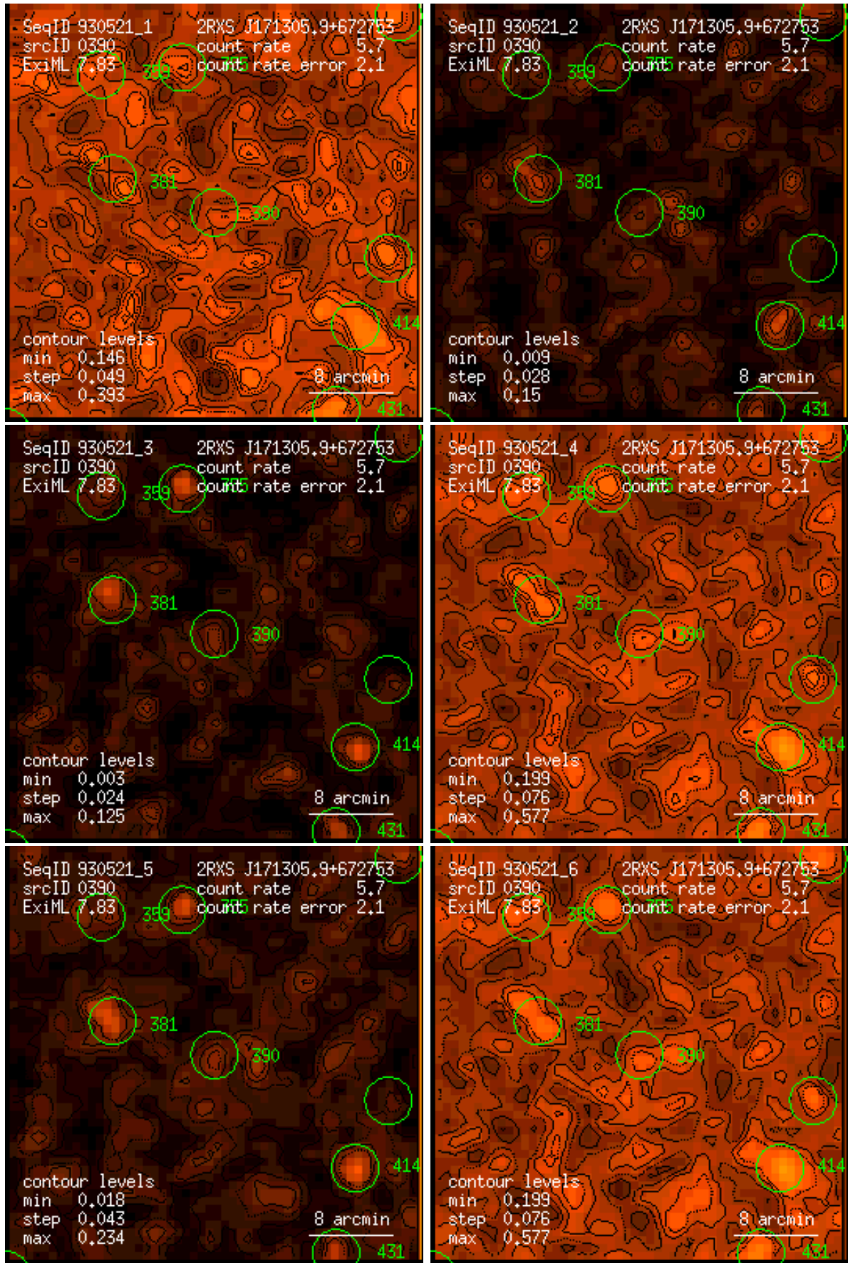
Figure 390: RASS 930521: detection 0390: band rate images, Gaussian filter: (1) PSPC channels 11 – 41, (2) 52 – 90, (3) 91 – 201, (4) 11 – 235, (5) 52 – 201, (6) 11 – 201. Broad band rates in counts/ks. Band rate contour levels in counts/ks/arcmin 2 .
