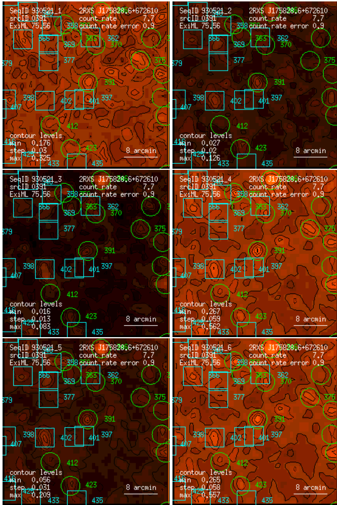
Figure 391: RASS 930521: detection 0391: band rate images, Gaussian filter: (1) PSPC channels 11 – 41, (2) 52 – 90, (3) 91 – 201, (4) 11 – 235, (5) 52 – 201, (6) 11 – 201. Broad band rates in counts/ks. Band rate contour levels in counts/ks/arcmin 2 .
