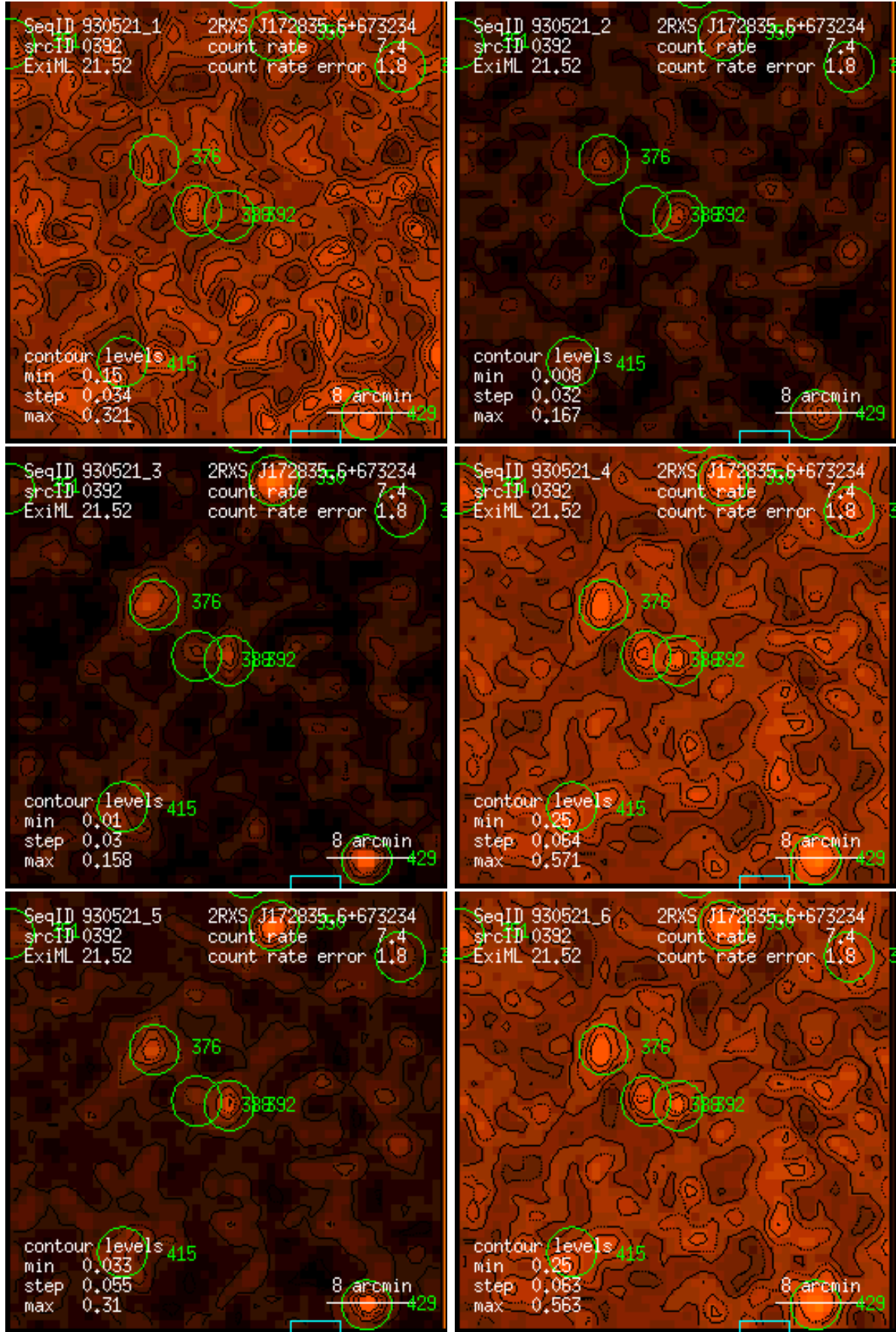
Figure 392: RASS 930521: detection 0392: band rate images, Gaussian filter: (1) PSPC channels 11 – 41, (2) 52 – 90, (3) 91 – 201, (4) 11 – 235, (5) 52 – 201, (6) 11 – 201. Broad band rates in counts/ks. Band rate contour levels in counts/ks/arcmin 2 .
