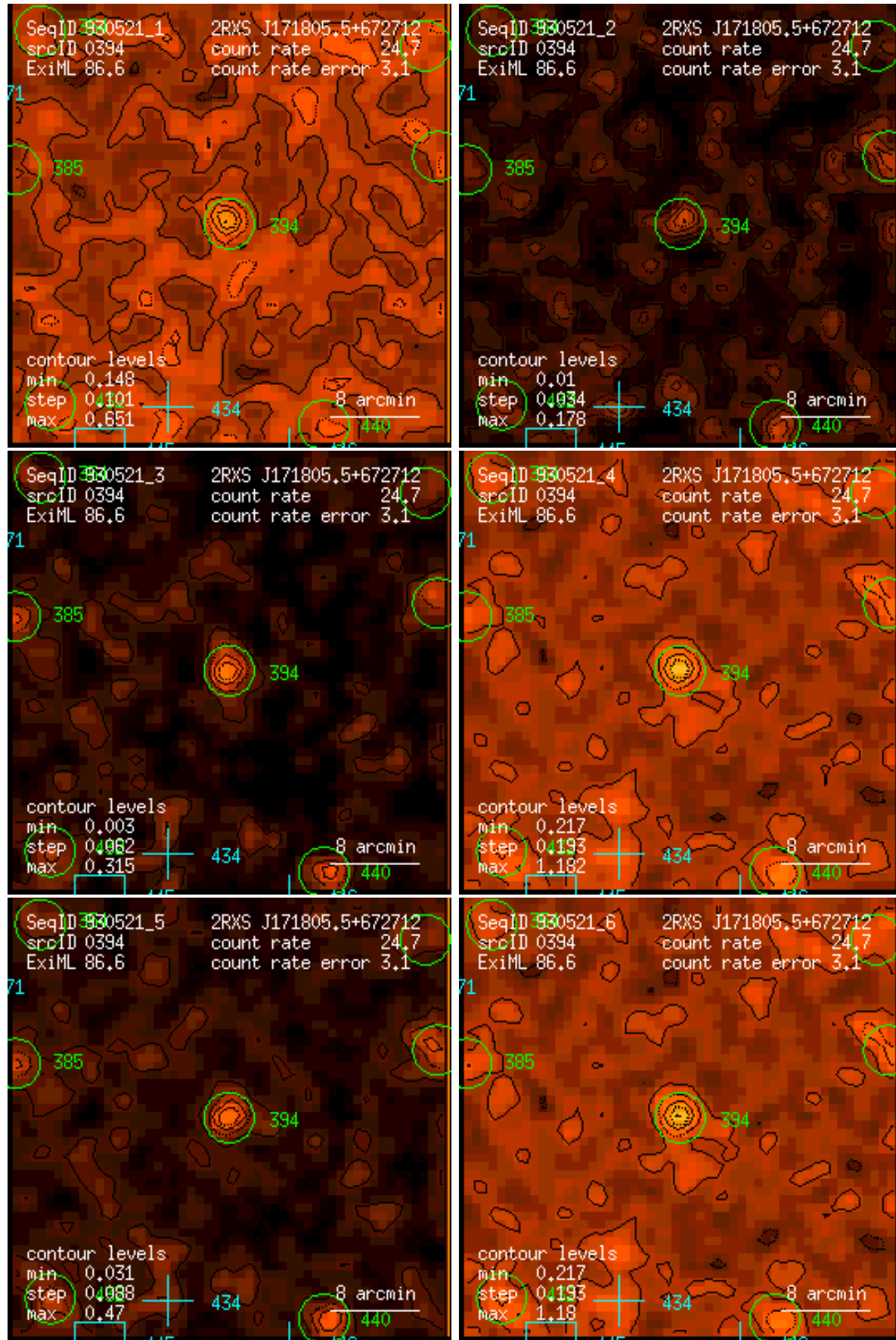
Figure 394: RASS 930521: detection 0394: band rate images, Gaussian filter: (1) PSPC channels 11 – 41, (2) 52 – 90, (3) 91 – 201, (4) 11 – 235, (5) 52 – 201, (6) 11 – 201. Broad band rates in counts/ks. Band rate contour levels in counts/ks/arcmin 2 .
