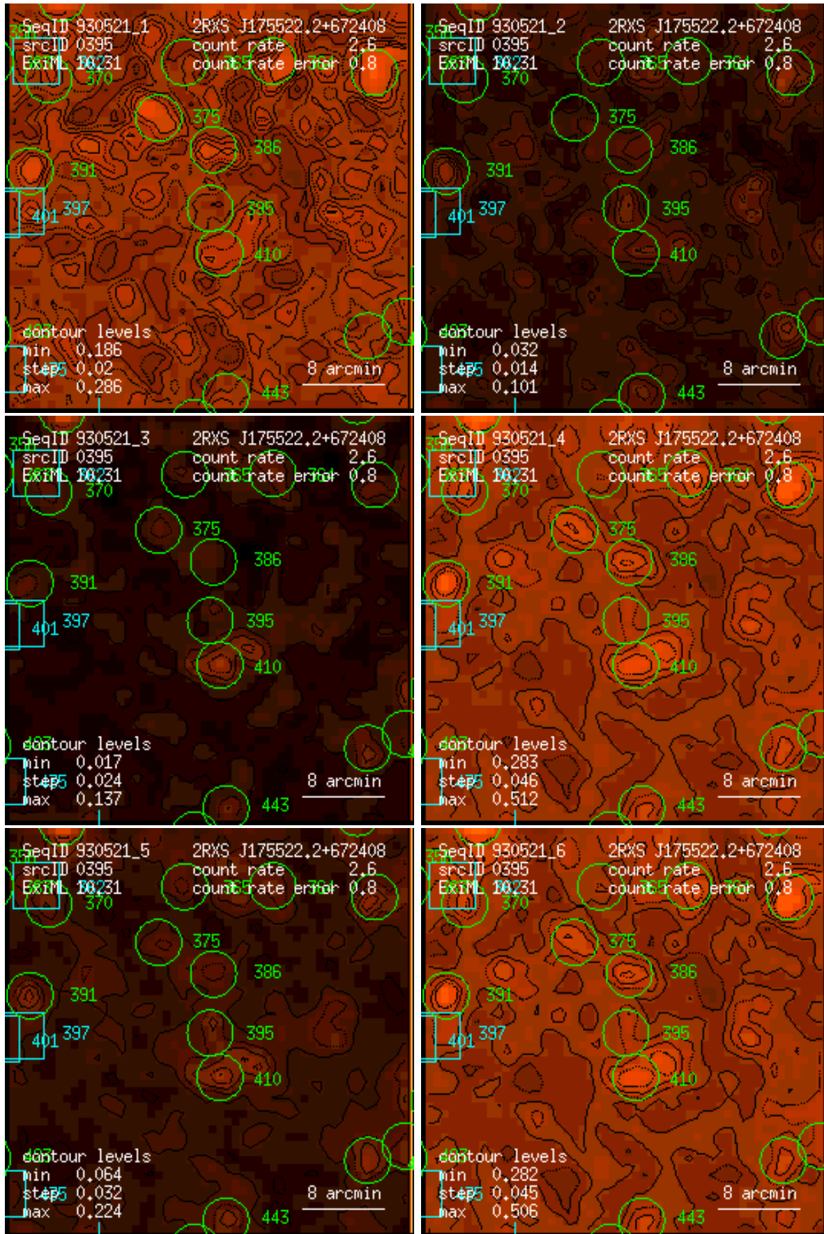
Figure 395: RASS 930521: detection 0395: band rate images, Gaussian filter: (1) PSPC channels 11 – 41, (2) 52 – 90, (3) 91 – 201, (4) 11 – 235, (5) 52 – 201, (6) 11 – 201. Broad band rates in counts/ks. Band rate contour levels in counts/ks/arcmin 2 .
