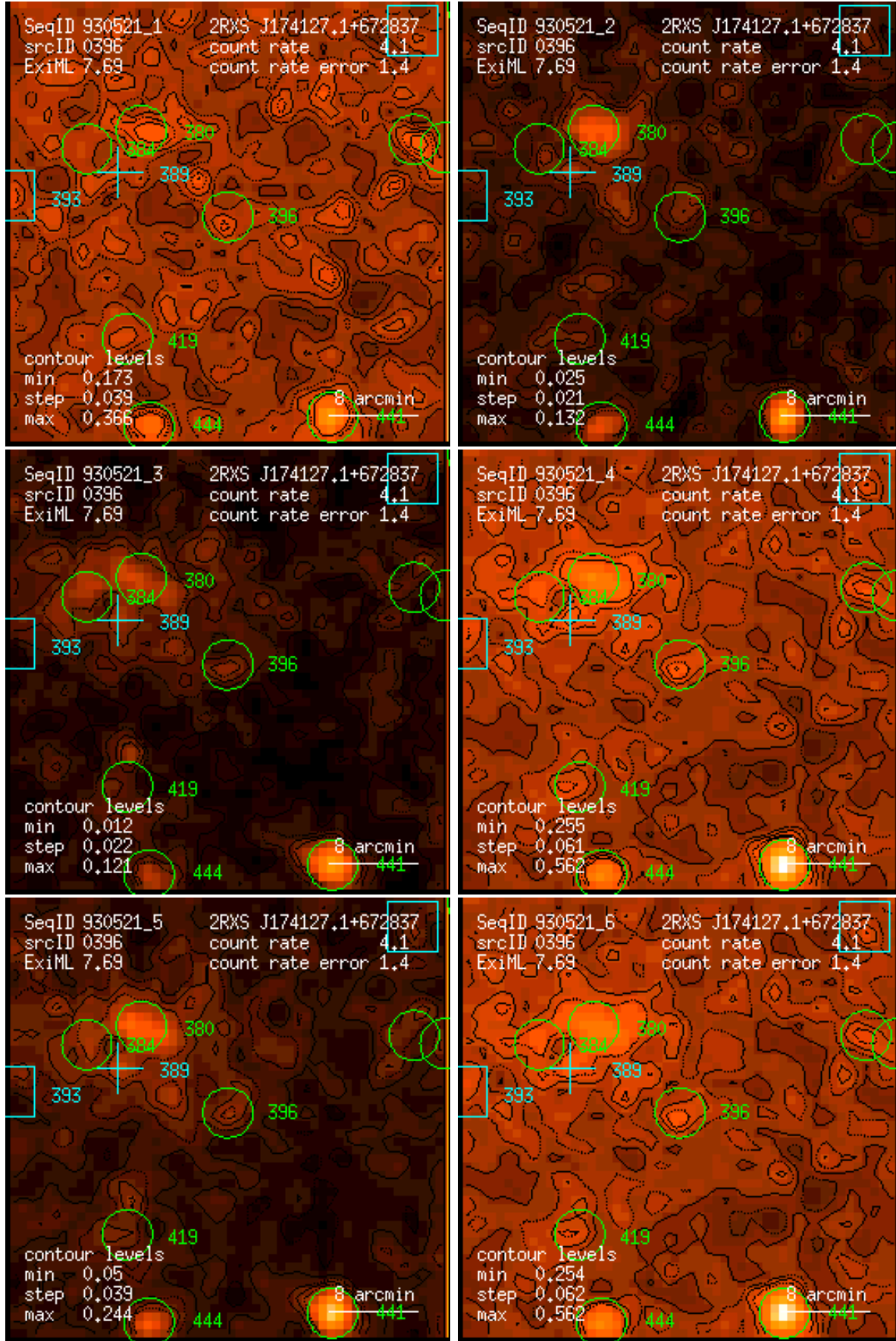
Figure 396: RASS 930521: detection 0396: band rate images, Gaussian filter: (1) PSPC channels 11 – 41, (2) 52 – 90, (3) 91 – 201, (4) 11 – 235, (5) 52 – 201, (6) 11 – 201. Broad band rates in counts/ks. Band rate contour levels in counts/ks/arcmin 2 .
