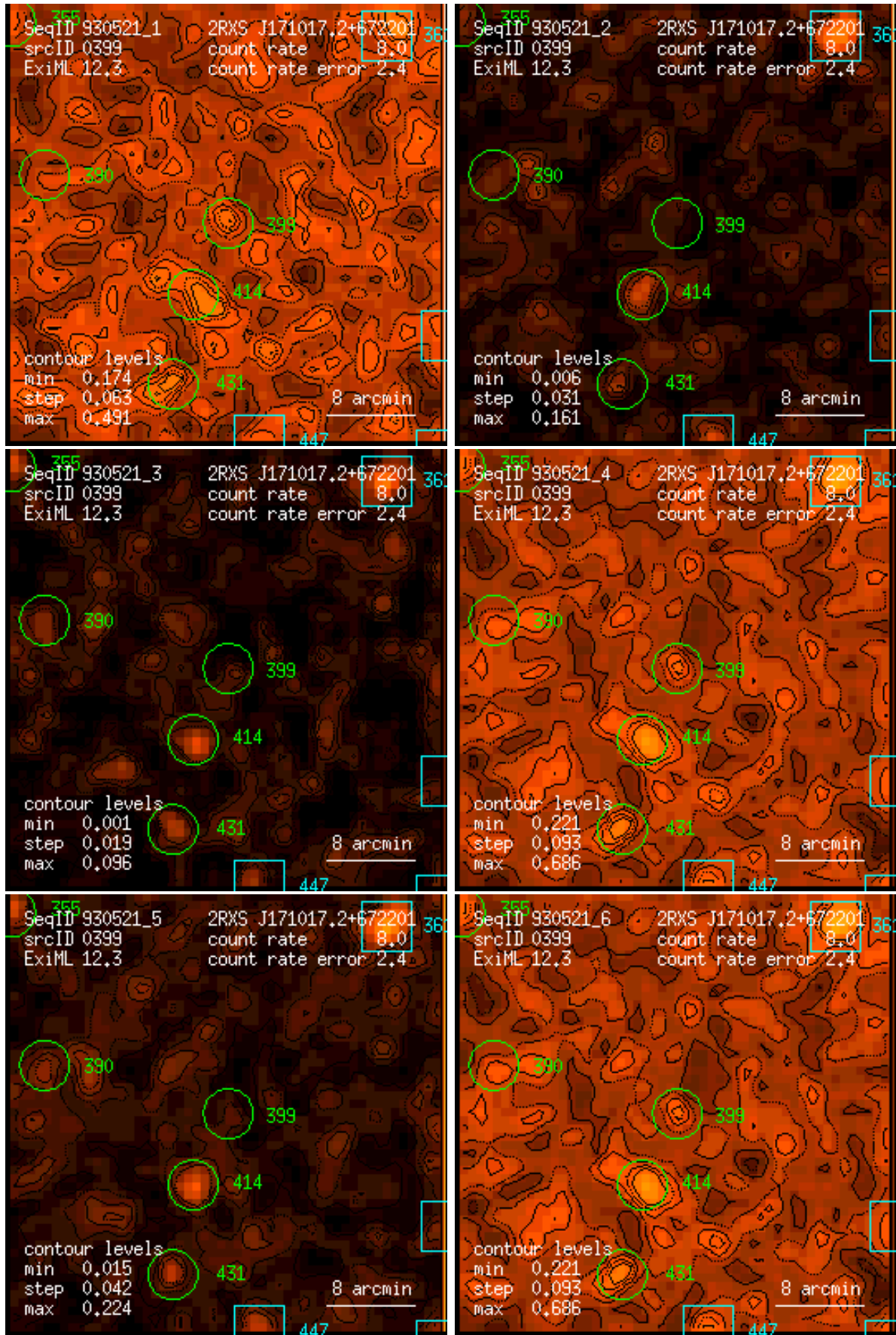
Figure 399: RASS 930521: detection 0399: band rate images, Gaussian filter: (1) PSPC channels 11 – 41, (2) 52 – 90, (3) 91 – 201, (4) 11 – 235, (5) 52 – 201, (6) 11 – 201. Broad band rates in counts/ks. Band rate contour levels in counts/ks/arcmin 2 .
