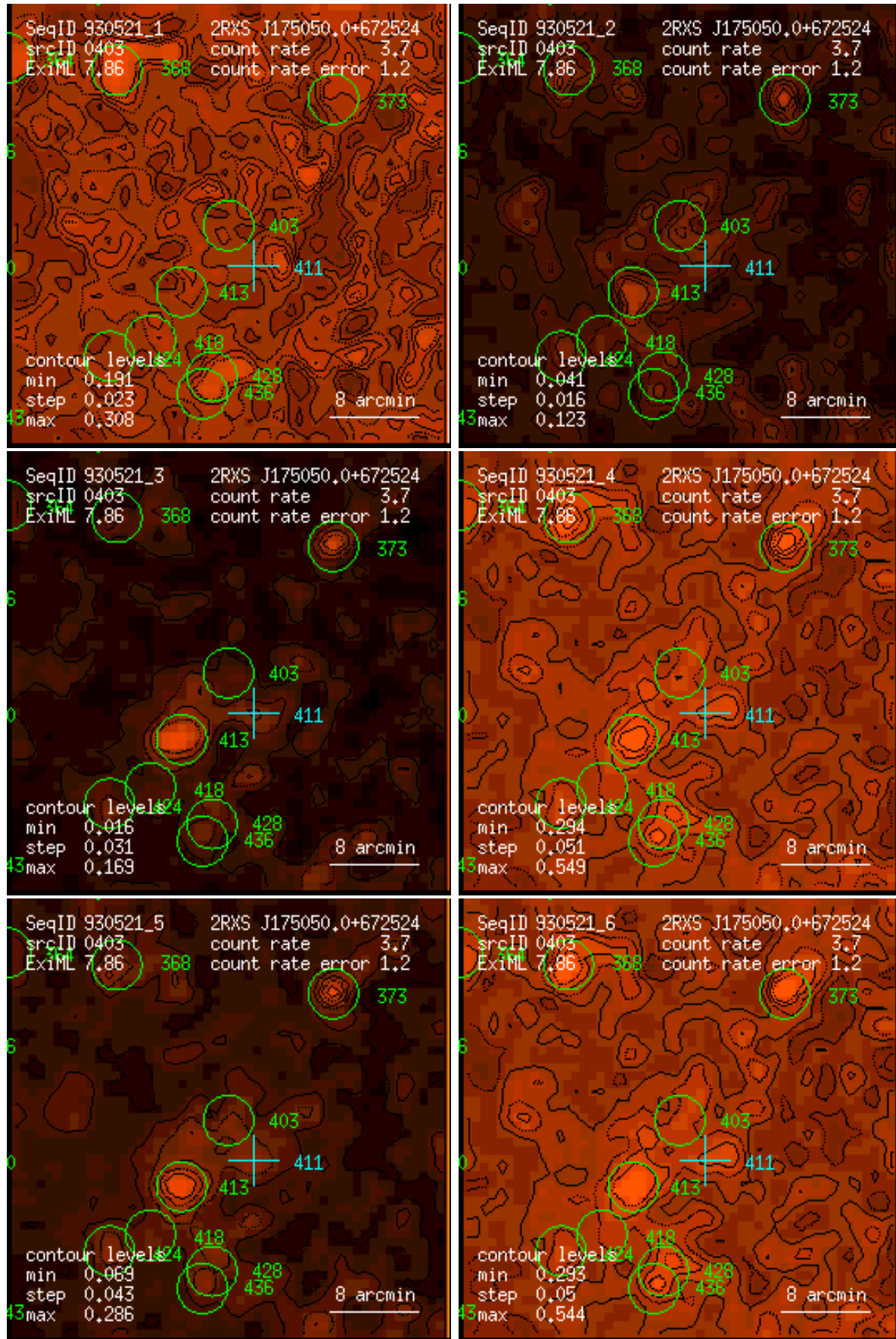
Figure 403: RASS 930521: detection 0403: band rate images, Gaussian filter: (1) PSPC channels 11 – 41, (2) 52 – 90, (3) 91 – 201, (4) 11 – 235, (5) 52 – 201, (6) 11 – 201. Broad band rates in counts/ks. Band rate contour levels in counts/ks/arcmin 2 .
