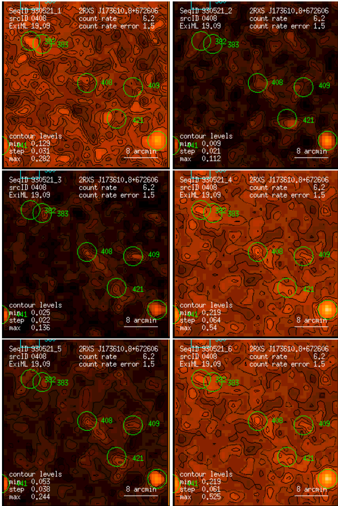
Figure 408: RASS 930521: detection 0408: band rate images, Gaussian filter: (1) PSPC channels 11 – 41, (2) 52 – 90, (3) 91 – 201, (4) 11 – 235, (5) 52 – 201, (6) 11 – 201. Broad band rates in counts/ks. Band rate contour levels in counts/ks/arcmin 2 .
