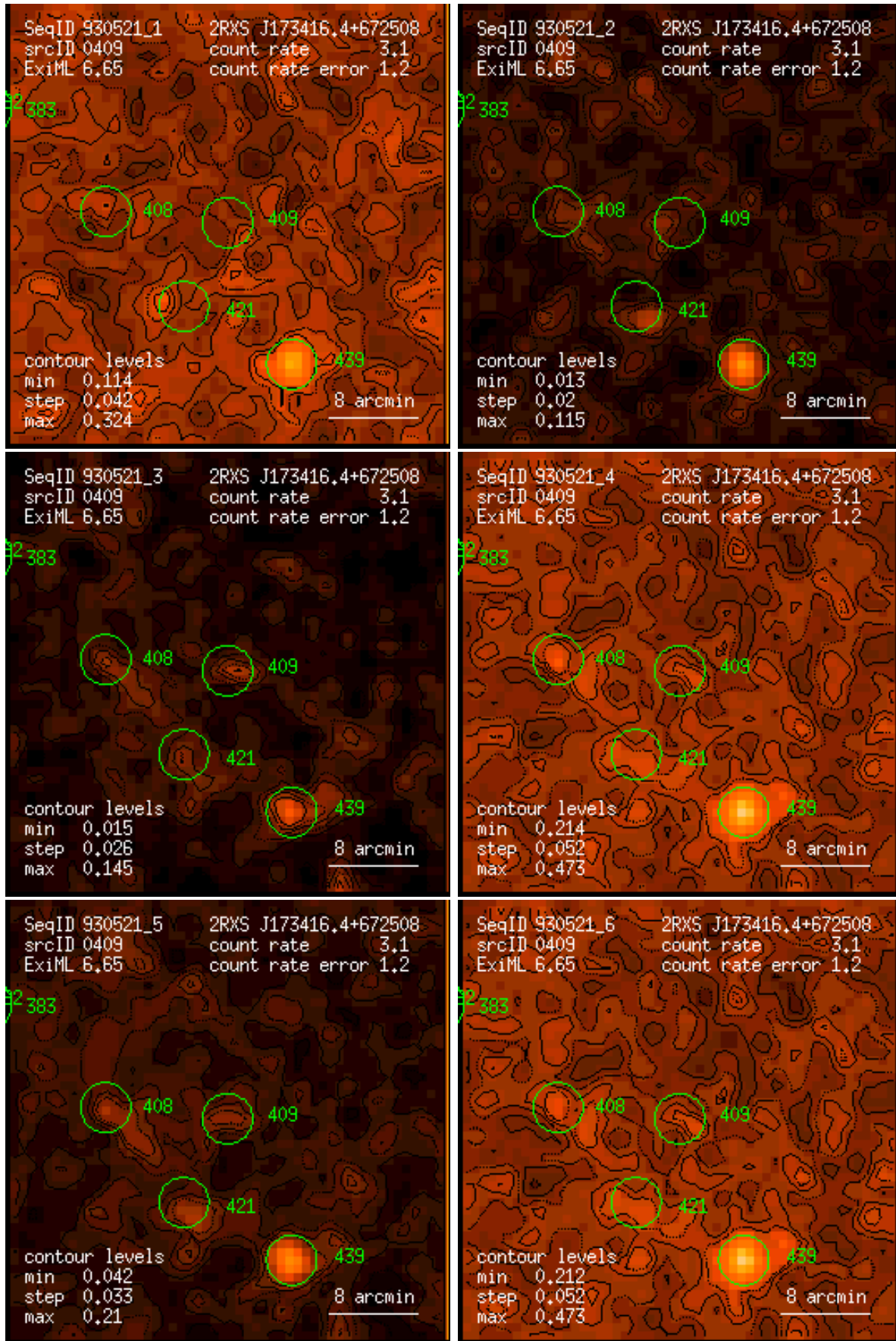
Figure 409: RASS 930521: detection 0409: band rate images, Gaussian filter: (1) PSPC channels 11 – 41, (2) 52 – 90, (3) 91 – 201, (4) 11 – 235, (5) 52 – 201, (6) 11 – 201. Broad band rates in counts/ks. Band rate contour levels in counts/ks/arcmin 2 .
